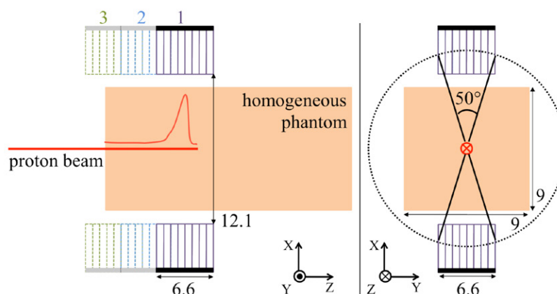
Figure 1. Top: photograph of the in situ TOF-PET setup at the HIT. The distance between the two detectors in the photograph is larger than in the actual measurement. Bottom: schematic overview of the measurement setup (not to scale), with distances displayed in centimeters. Three longitudinal detector positions with FOV overlaps of 2.5 cm covered the full proton beam range. This was accomplished by translating the phantom over its support rail.
