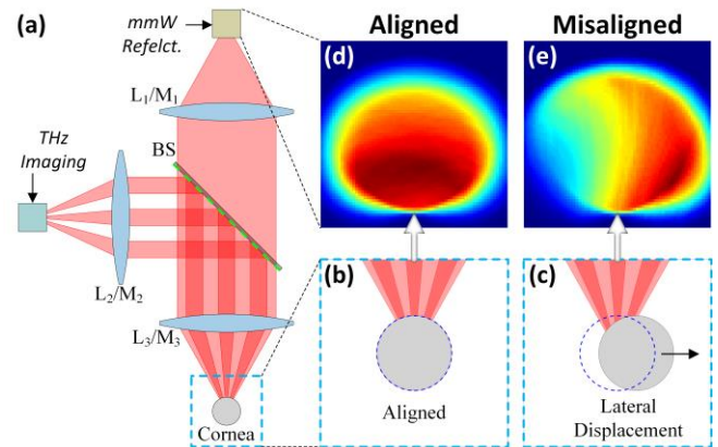
Figure 1. Alignment concept. (a) A quasi-optical duplexer (e.g. wire grid polarizer) multiplexes the THz and mmW beams on a common optical axis. When the cornea is positioned correctly with respect to the aperture in (b) the THz image shows the contrast in (d). When the cornea is misaligned (c) there is a significant change in imaging contrast (e) arising from the rapid degradation in coupling.
