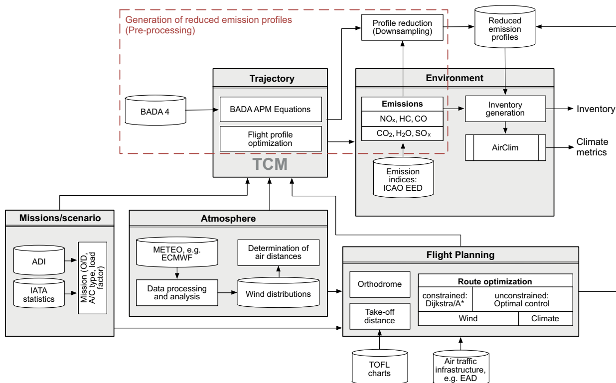
Figure 1: Schematic diagram of the developed modeling system (abbreviations: A/C – aircraft; O/D – origin/destination; see text for further acronyms).
