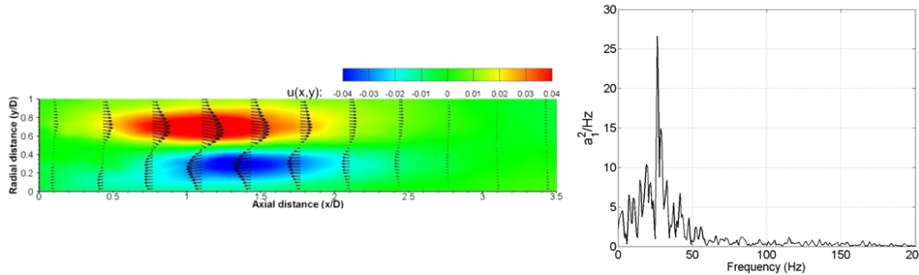
Figure 6: The first POD spatial mode (left) and the spectrum of the corresponding temporal mode (right)
