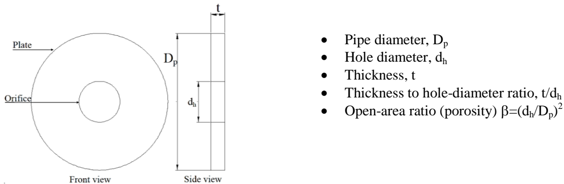
Figure 1: Geometry of sharp-edged single-hole orifice and nomenclature
