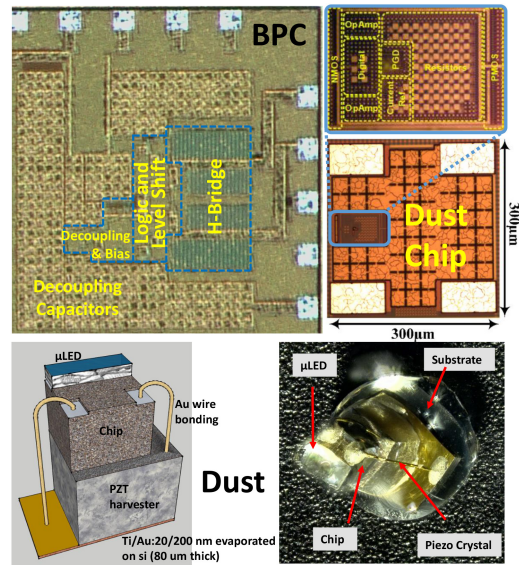
Fig. 6. Die micrograph of BPC and Dust cores, Dust integration strategy, and integrated Dust prototype.
