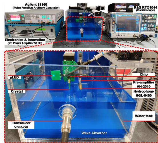
Fig. 11. Measurement setup for testing the entire system.
