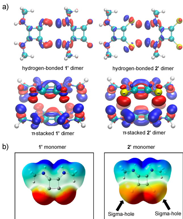
Figure 8. (a) Computed electron density difference (EDD) maps for the head-to-tail 1' and 2' dimers (note the larger lobes on 1' ), as well as stacked 1' and 2' dimers (note the larger lobes on 2' ). (b) Electrostatic potential maps (MEP) of 1' and 2' monomers (blue indicates electron density loss and positively charged; red indicates electron density gain and negatively charged).
