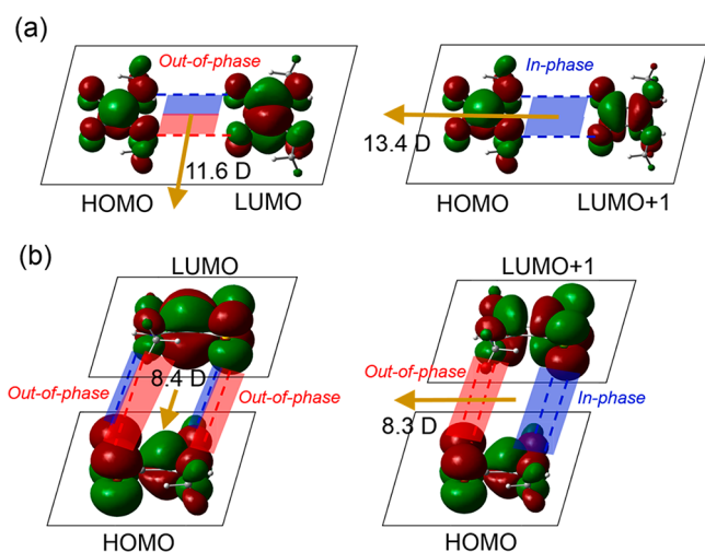
Figure 4. Orbital interactions of neighboring monomers in HOMO–LUMO and HOMO–LUMO+1 transitions for (a) head-to-tail (for 1') and (b) stacked (for 2') arrangements. The direction and magnitude of the computed transition dipole moments for each transition are indicated.
