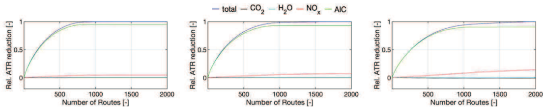
Figure 3. Cumulative ATR reduction as a function of the number of changed routes for 1% (left), 2% (middle) and 14.5% (maximum) increase in fuel burn (right) for the top 2,000 routes. Individual contributions to the total ATR reduction (blue) are shown for CO 2 (black), H 2 O (cyan), NO x (red) and contrails (green).
