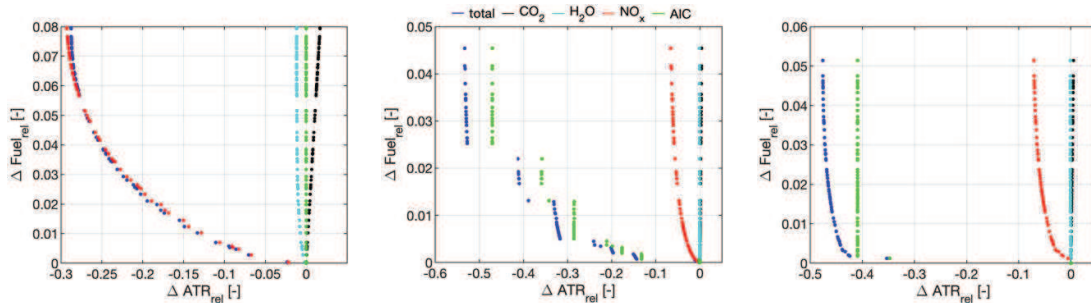
Figure 1. Pareto-fronts for Baku-Luxembourg (left) Lulea-Gran Canaria (middle) Helsinki-Gran Canaria (right). The coloured dots indicate the individual contribution of \text{CO}_2 (black), \text{H}_2\text{O} (cyan) \text{NO}_x (red) and contrails (green) to the overall climate impact reduction (blue) for a given fuel increase. Results are expressed relative to the minimum fuel case.
