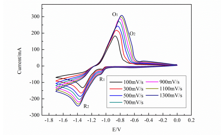
Figure 3. Cyclic voltammograms of the LiCl-KCl-K 2 ZrF 6 (1 wt%) system with varied scan rates at 550 °C.
