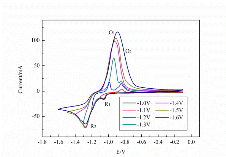
Figure 2. Cyclic voltammograms of the LiCl-KCl-K 2 ZrF 6 (1 wt%) system at 550 °C with the scan rate of 100 mV/s in varied scan ranges.
