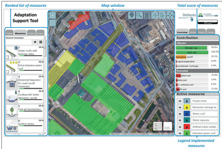
Figure 10. Adaptation Support Tool interface with three panels. The left panel includes the project set-up, the list of measures from the tool's library, and additional layers. The map window is where measures are implemented from the list. The right panel includes the quantitative indicators of the costs and effectiveness of the applied measures, detailed impacts per measure and the adaptation targets.
