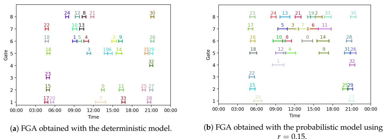
Figure 10. Flight-to-gate assignments for 14 July 2019 obtained using the deterministic and probabilistic models.
