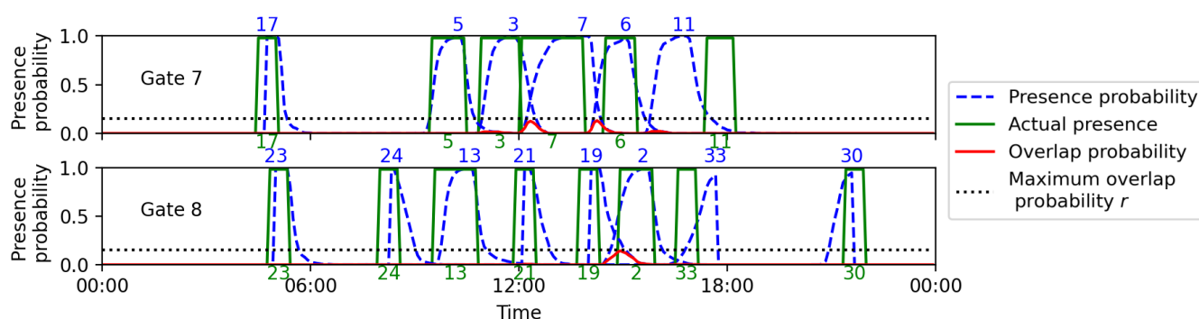
Figure 11. Flight-to-gate assignment for gates 7 and 8 on 14 July 2019 obtained using the probabilistic model with maximum overlap probability r = 0.15 combined with actual aircraft presence.
