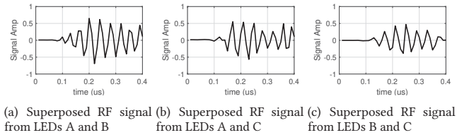
Figure 10: Observation 2: the superposed side-channel RF signals from multiple LEDs are also unique from each other.
