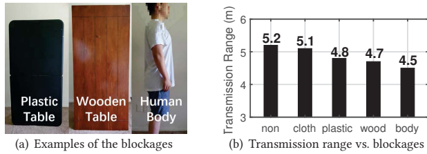
Figure 22: Evaluation with different blockages: (a) Examples: plastic, 2 cm wooden table, and a human body; (b) Results.
