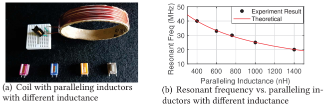
Figure 6: Experiment with paralleling inductors.
