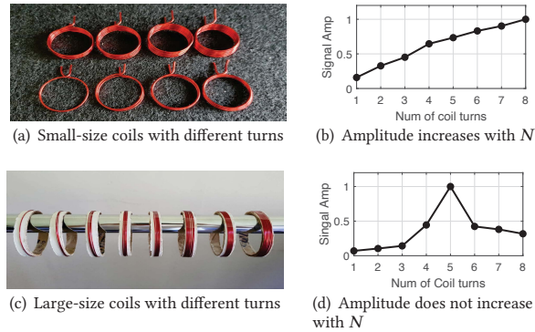
Figure 4: Validating the impact of coil turns on side-channel signal amplitude: (a-b) small coils (diameter: 2.6 cm) and the results; (c-d) large coils (diameter: 7.8 cm) and the results.
