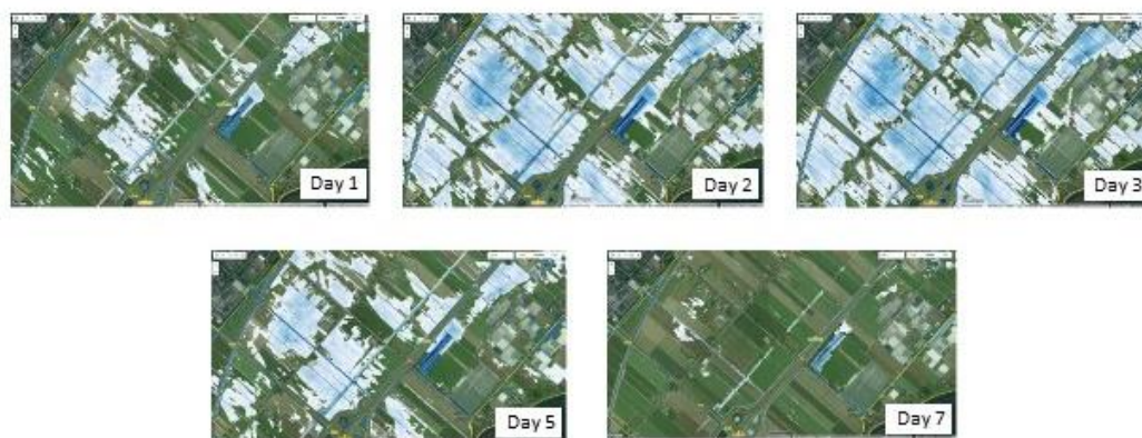
Figure 3: Time evolution of surface water in a spatial section of the “Haarlemmermeer” at day 1, day 2, day 3, day 5 and day 7 of the projected rainfall event (De Bruijn & Slager, 2021).
