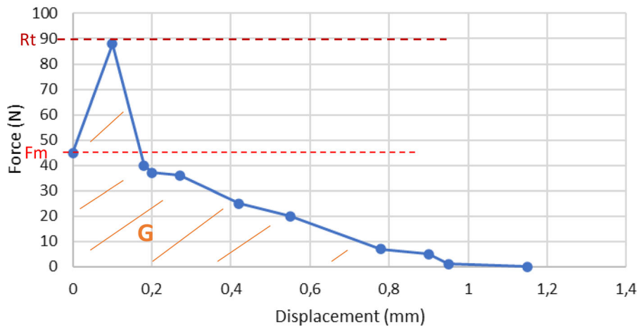
Fig. 13 Force–displacement curve of a tensile test after a restrained shrinkage test for a lime-metakaolin mortar (lime-MK:sand volumetric proportions 1:0, 10:3) with indication of G (rupture energy) [51]
