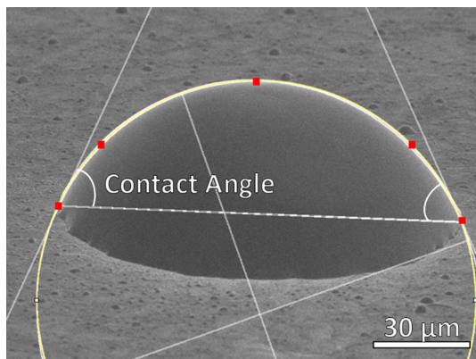
Fig. 6—SEM image of Pb droplets on Fe–1.9 Mn–0.94 Si steel annealed at DP -40\text{ }^{\circ}\text{C} . The sample surface normal is tilted by 70\text{ }^{\circ} deg with respect to the electron beam. The red squares indicate the selected points on the contour line of the Pb droplet for image analysis, the yellow curve indicate the ellipse used to fit the contour line (Color figure online).
