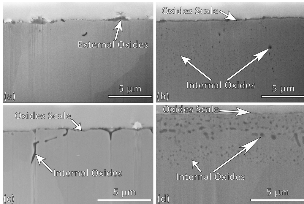
Fig. 5—SEM images of the cross-section of Fe–1.8 Mn steel annealed at dew points (a) -40\text{ }^{\circ}\text{C} and (b) +10\text{ }^{\circ}\text{C} ; and Fe–1.9 Mn–0.94 Si steel annealed at dew points (c) -40\text{ }^{\circ}\text{C} and (d) +10\text{ }^{\circ}\text{C} for 1 h at 950\text{ }^{\circ}\text{C} in a mixture of Ar + 5 vol pct \text{H}_2 .
