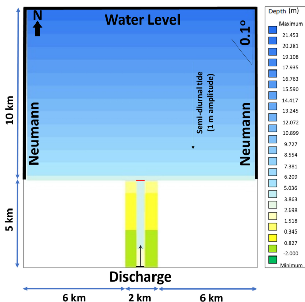
FIGURE 2 The model setup consists of a channel debouching into a sloped basin with a 0.1° gradient. The boundary condition at the channel inflow (horizontal thin black line) is water and sediment discharge, whereas the open boundaries in the basin (horizontal and vertical thick black lines) are the Neumann at the west and east combined with water level along the north boundary. The initial water depth ranges from 4 m at the delta apex (horizontal thin red line) to 21.5 m at the basin edge.
