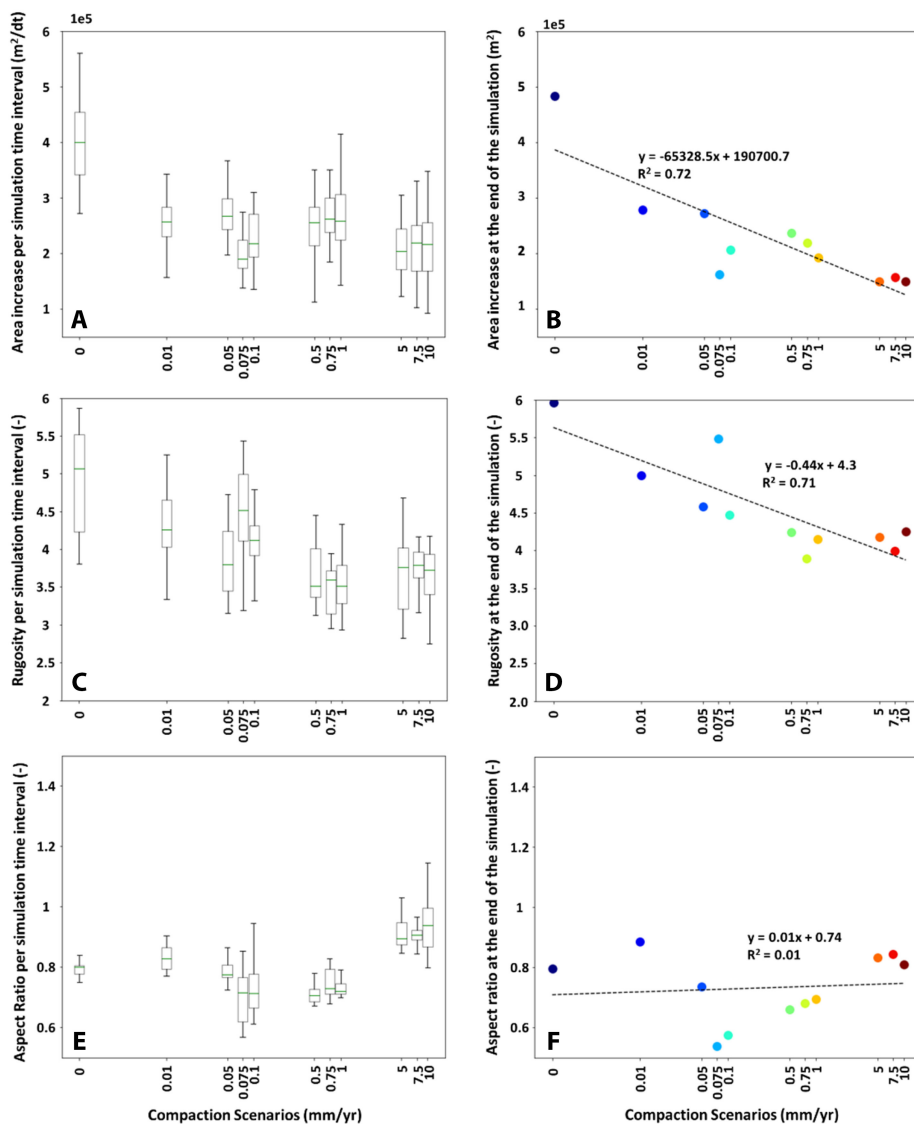
FIGURE 6 The first column shows box plots, which indicate a collapse time series of the area increase, rugosity and aspect ratio for mud-rich deltas with compaction scenarios ranging from 0 to 10 mm year -1 (A, C and E). Each box plot shows a median value (second quartile, horizontal green lines) between the first and third quartiles (interquartile range, grey boxes). The vertical black lines indicate the maximum and minimum data range. The second column indicates the area increase, rugosity and aspect ratio at the end of the simulation, accounting for temporal variation of morphology trends (B, D and F). Trendlines with linear equations and coefficient correlations are also included for each morphology trend. Note that the x-axis is in the log scale.
