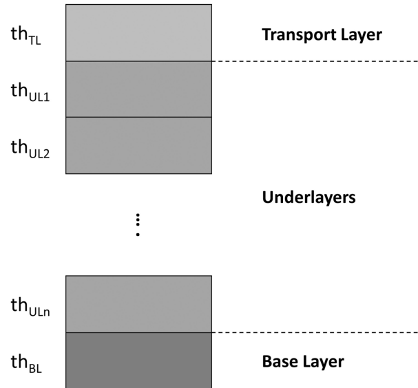
FIGURE 1 Multi-layer administration in Delft3D, consisting of a transport layer, n numbers of underlayers, and a base layer. The transport layer has a fixed thickness of 0.2 m ( th_{TL} ). Seventy five underlayers were used in the simulation ( th_{UL} ), each having a maximum thickness of 0.3 m. The base layer has a flexible thickness ( th_{BL} ).
