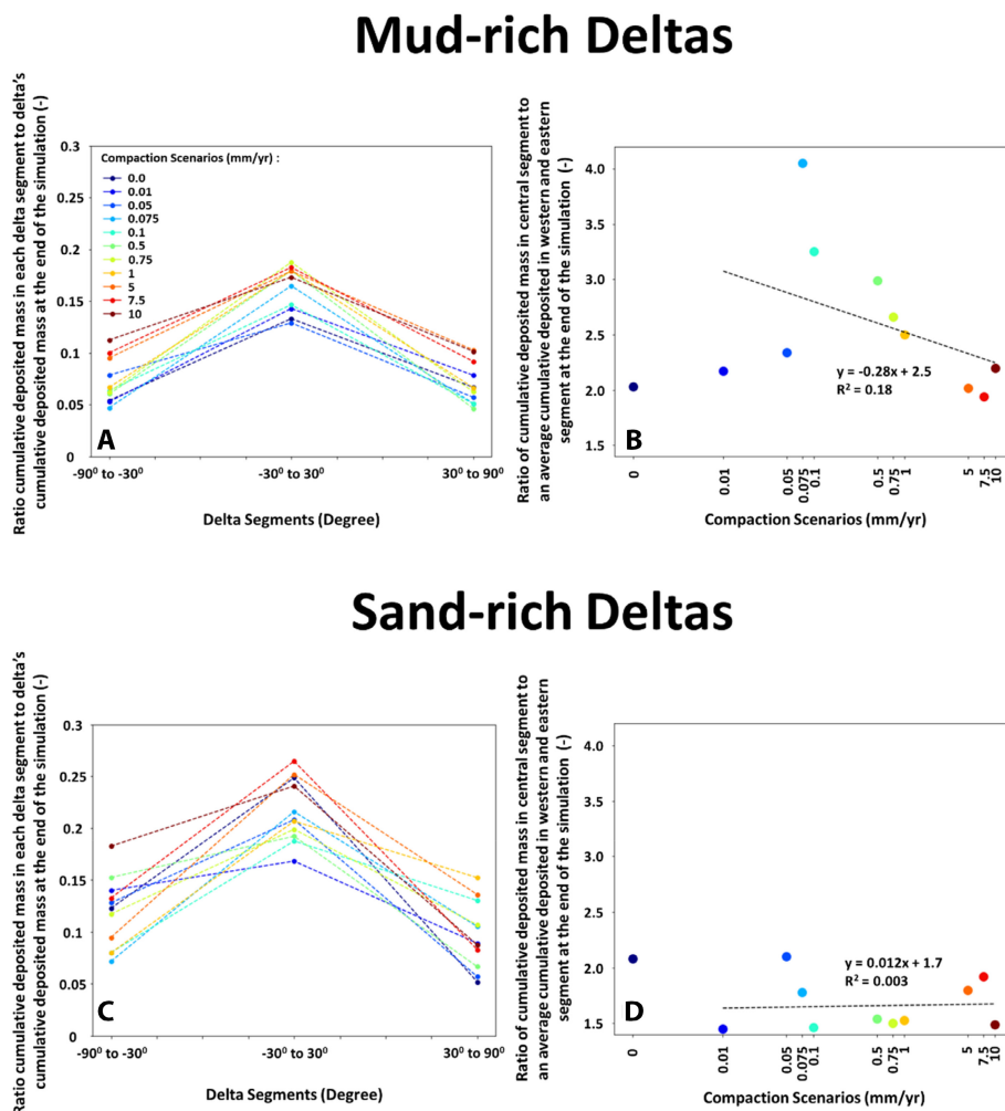
FIGURE 8 The left hand figures indicate the distribution of deposited sediment alongshore, shown by the ratio of cumulative deposited mass in each delta segment ( -90^\circ to -30^\circ , -30^\circ to 30^\circ and 30^\circ to 90^\circ ) and the delta's cumulative deposited mass at the end of the simulation for mud-rich and sand-rich deltas (A and C). To show how evenly the deposition occurs alongshore, the ratio of cumulative deposited mass in the delta centreline ( -30^\circ to 30^\circ ) is calculated to an average of two side segments ( -90^\circ to -30^\circ and 30^\circ to 90^\circ ) at the end of the simulation, shown in the right hand figures for mud-rich and sand-rich deltas (B and D). Trendlines with linear equations and coefficient correlations are also included. The calculation of delta segments is explained in Section 4.2. Different coloured lines and dots indicate compaction scenarios, from 0 to 10 mm year -1 .
