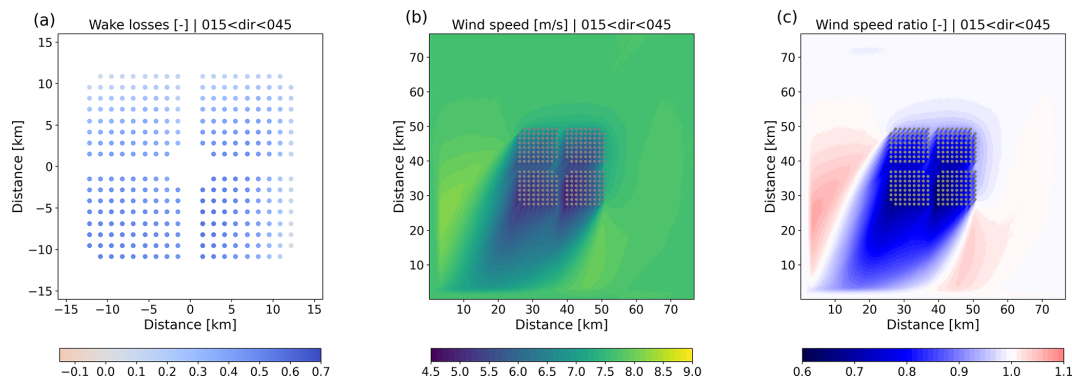
Figure 19. Same as Fig. 13 but only including stable conditions, wind speeds between 6 and 10 \text{ m s}^{-1} , and wind directions between 15 and 45^\circ .
