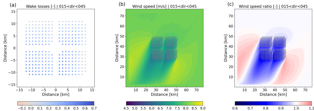
Figure 18. Same as Fig. 13 but only including convective conditions, wind speeds between 6 and 10 \text{ m s}^{-1} , and wind directions between 15 and 45^\circ .
