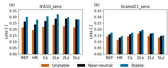
Figure 21. Stability-dependent aerodynamic losses for disk-averaged wind speeds between 6 and 10 \text{ m s}^{-1} for the IEA10 (a) and Scaled21 (b) sensitivity experiments.
