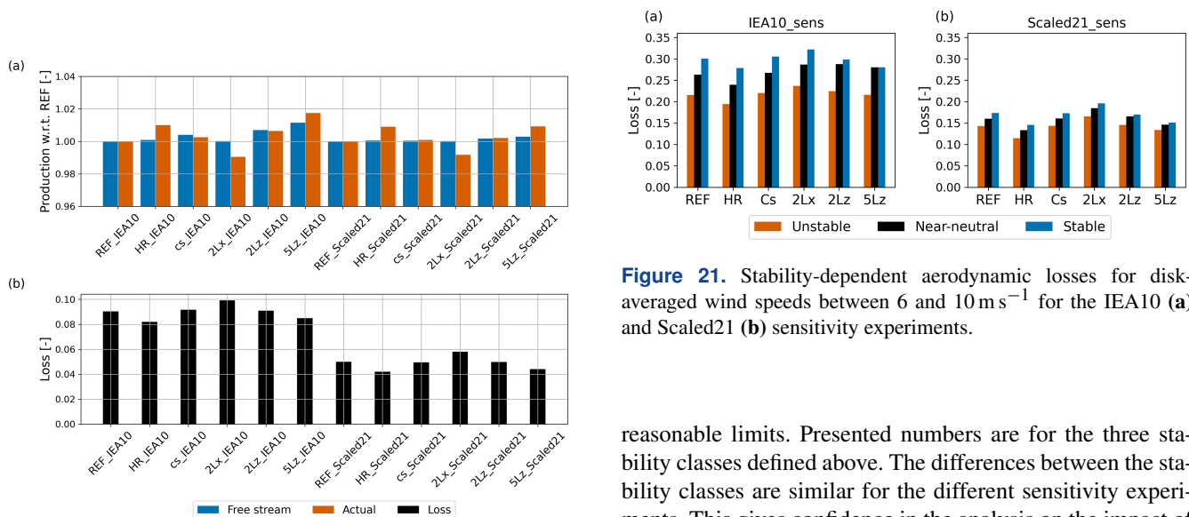
Figure 20. Free-stream and actual production of the sensitivity experiments with respect to REF (a) and the corresponding aerodynamic losses (b).
