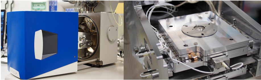
Figure 2.3: Photographs of the integrated fluorescence and electron microscope system. Left: Verios SEM (vacuum chamber visible on the right) retrofitted with a wide-field optical microscope. The sample stage is attached to the blue-boxed vacuum door with a fluorescence camera. Right: A closer view of the sample stage (x-y movement) and the optical objective stage (z-movement) below this. A representative sample on an Indium Tin Oxide (ITO)-coated glass coverslip is shown, mounted on an Aluminium sample holder ring.
