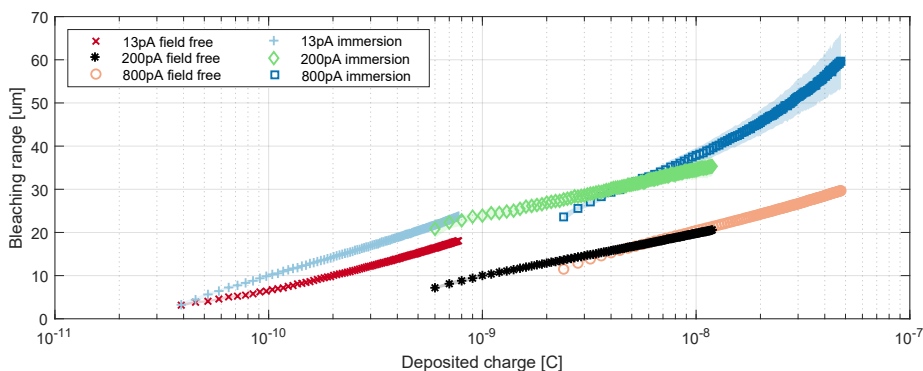
Figure 5.7: Bleaching range as a function of deposited charge for field-free and immersion SEM lens modes for 13, 200, and 800pA currents. For the immersion mode, all data points lie approximately on one line, whereas the field-free mode shows a difference between the low (13pA) and high currents (200 and 800pA).
