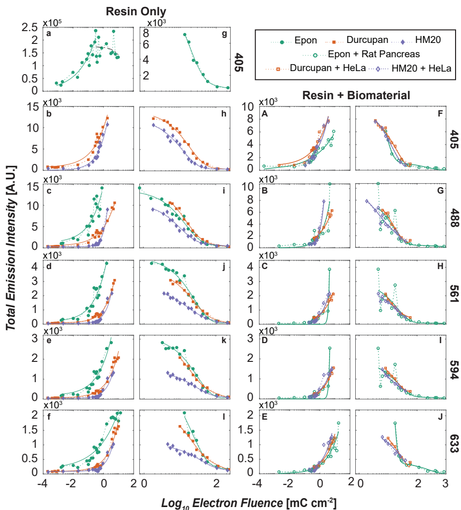
Figure 3.9: Total emission intensity as a function of electron fluence for bare (a-l) and bio-embedded (A-J) resins and corresponding fit curves. The associated excitation wavelength is denoted on the right of each row panel. (a-f) and (A-E) separate the rising intensity regime from the decay in (g-l) and (F-J). Dotted lines and solid lines represent experimental data and fit curves, respectively. Filled and open markers are used to distinguish bare and bio-embedded data. The black dashed line for bare Epon at 405nm denotes data outliers to the applied fit equations. Displayed in semi-logarithmic scale. Rising curves are fit to a power law; decay curves are fit to a double exponential. HM20 has the slowest rise curves in the bare resins. Embedding biomaterial reduces intensity differences.
