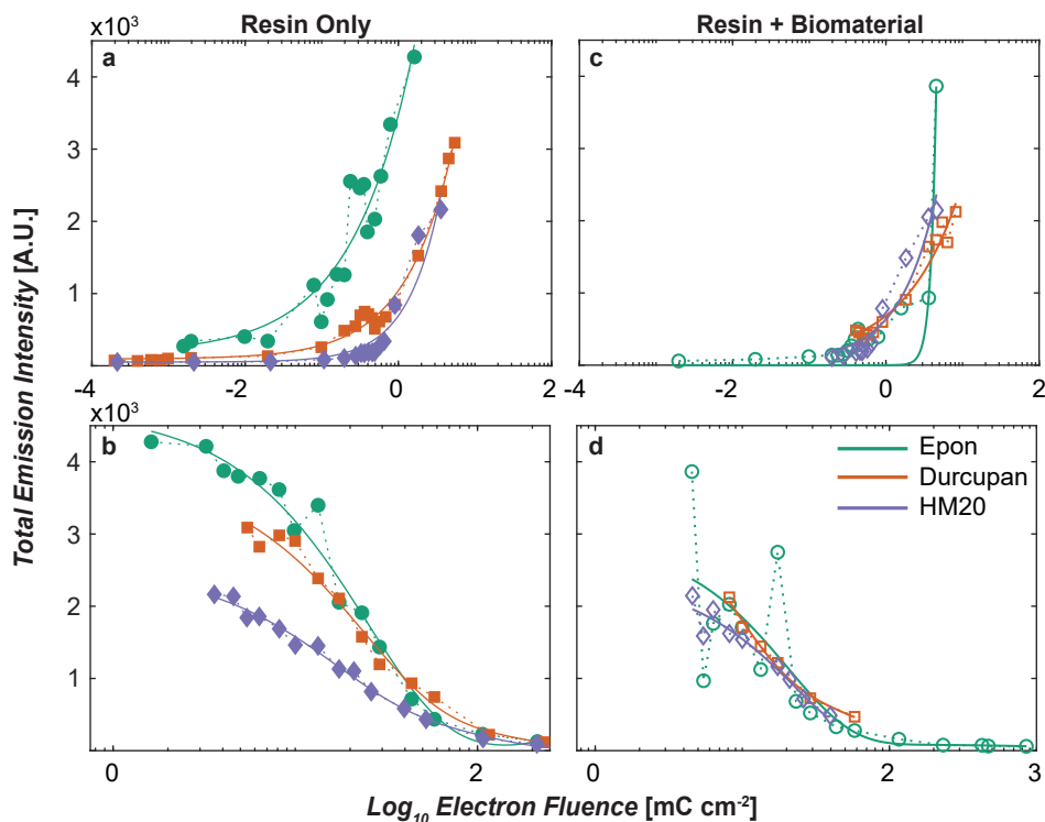
Figure 3.4: Luminescence rise and bleaching curves fall in similar fluence magnitude regimes across samples. (a) The rise in electron-induced luminescence for all bare resins is shown (excitation: 561nm) as a function of electron fluence. (b) The decay in luminescence in the bleaching regime. (c-d) Similar curves for the resins with embedded biomaterials. Symbols indicate measured values; solid lines indicate fit with a power-law and double-exponential function for the rise and bleaching regime, respectively. In all cases, the induced luminescence rises between 10^{-3} and 5 \text{ mC cm}^{-2} , and decays between 5 and 100 \text{ mC cm}^{-2} . Full curves for all excitation wavelengths and materials can be found in the supporting information later in this chapter.
