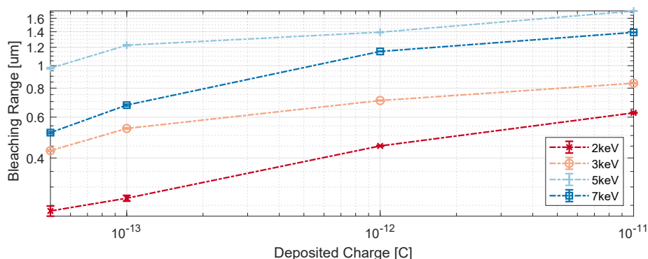
Figure 5.11: Bleaching range as a function of deposited charge for a plastic scintillator. Row 1 as seen in Figure 5.10 is not depicted due to a low signal-to-background ratio.
