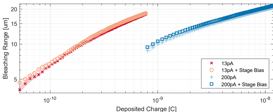
Figure 5.9: Bleaching range as a function of deposited charge shows that the former is independent of an applied -500V stage bias. The graphs represent 13pA and 200 pA currents for a system with and without a -500V stage bias. The effective landing energy was maintained at 1keV in both cases.
