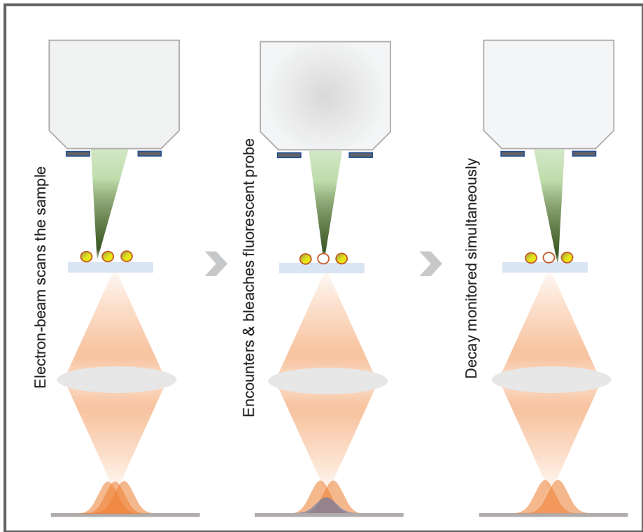
Figure 2.2: Illustration of the eSRM principle. A sample with active fluorescence labels (depicted as yellow spheres) is mounted in an integrated fluorescence (orange) and electron (green) microscope. Each label on the pixelated fluorescence detector (at the bottom) gives a Gaussian-shaped image; the sum of all illuminated labels constitutes the diffraction-limited image. Electron exposure of a specific label during scanning leads to bleaching of that label (middle panel), resulting in a localized decay in fluorescence on the detector. Synchronization of the detected fluorescence loss with the electron beam's instantaneous position allows sub-diffraction limit localization of the fluorescence label.
