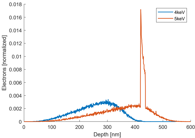
Figure 5.6: Normalized histogram depicting the maximum penetration depth of primary electrons at 4 and 5keV landing energy, using CASINO v2.3. Our sample scheme served as the input to the simulation with a 440nm layer of fluorescent perylene diimide on a 10nm ITO-coated glass substrate. The graphs depict the maximum depth traveled by an incoming electron at 4 or 5keV before it loses enough energy to halt in the material. At 4keV, the electrons stop in the perylene layer, while at 5keV landing energy, most scatter in the ITO layer. This is evident from the peak at 450nm due to the higher ITO density compared to that of perylene.
