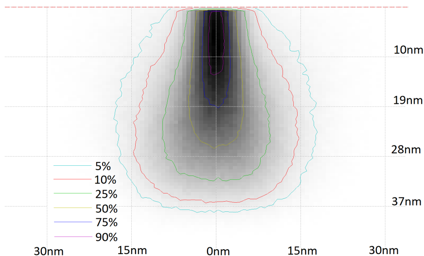
Figure 5.2: Energy deposition of 10^5 electrons in a Polymethylmethacrylate-ITO-glass substrate (CASINO v2.3 simulation). See main text for details on individual material thicknesses. The lines depict the distance at which a percentage of the incoming electron energy is deposited. The electrons' penetration depth and transverse spread are \sim 40 nm and \sim 30 nm, respectively. This is considerably smaller than that observed later in Figures 5.3a to 5.3d.
