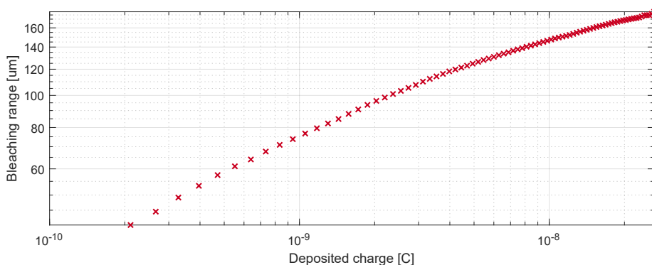
Figure 5.12: Bleaching range increases ten-fold in the presence of aluminum oxide. 1keV focused electron-beam irradiation of bulk perylene spin-coated on a 10nm aluminum oxide layer on ITO-coated glass. The bleaching range is depicted as a function of deposited charge for a 13pA current. Strong insulating properties of aluminium oxide result in a ten-fold increase in bleaching range for similar deposited charges as seen in Figure 5.7. The key difference is that an electrical insulator is now placed between the fluorescent layer and the conductive ITO.
