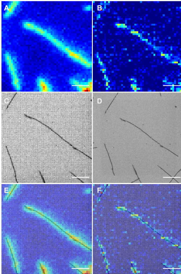
Figure 2.8: eSRM applied to fluorescently labeled microtubules. (A) WF fluorescence image of microtubules labeled with TRITC. (B) eSRM, (C) RT-SEM, and (D) high-resolution SEM images of the same microtubules, (E) WF, and (F) eSRM fluorescence overlays with RT-SEM, respectively. Scale bar 1\mu\text{m} .
