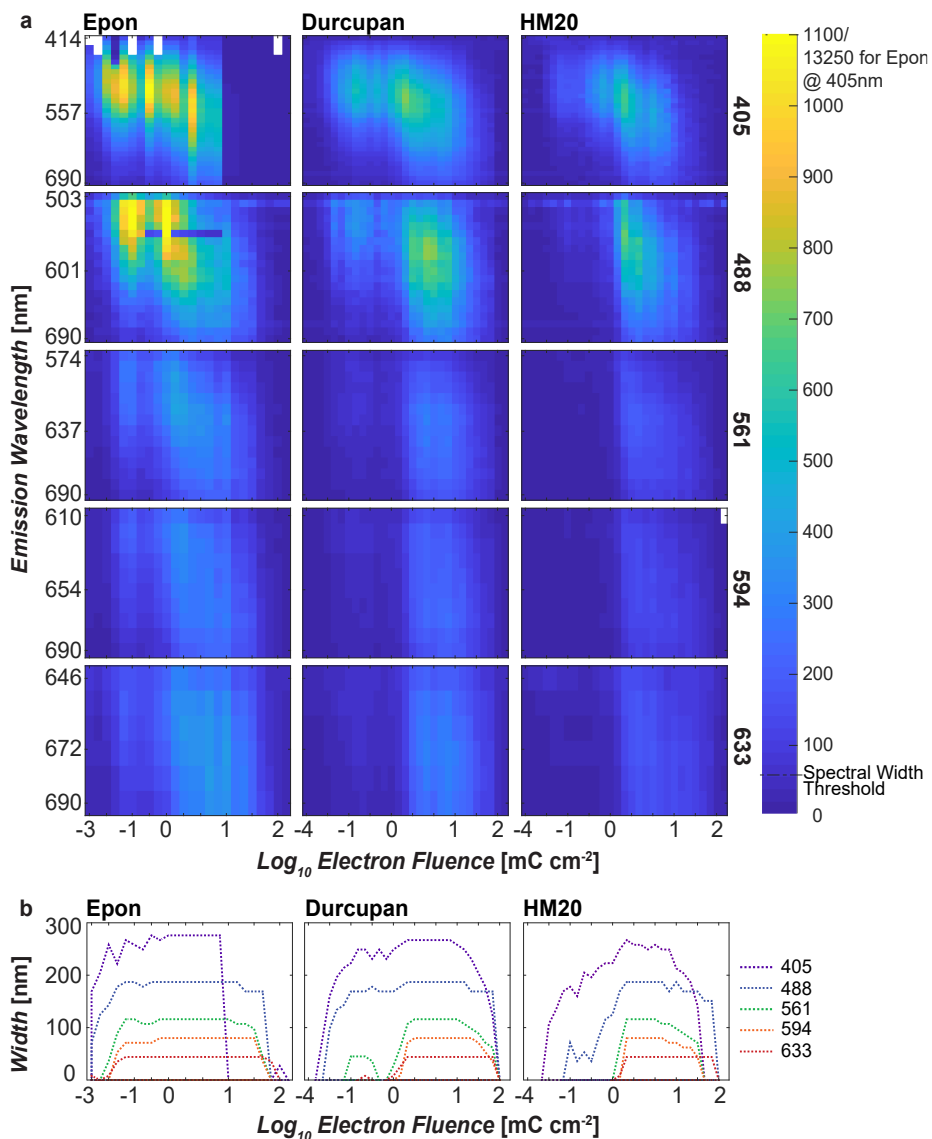
Figure 3.5: Electron-induced luminescence spectrum shifts from blue to red upon increasing electron fluence. (a) Color-coded luminescence emission intensity as a function of electron fluence for each of the different excitation wavelengths indicated on the right. White pixels denote missing values. (b) Spectral width as a function of electron fluence for each excitation wavelength and resin. The spectral width has been defined as the range in which the threshold intensity indicated in the color scale in (a) is exceeded. The threshold (725 for bare Epon and 60 units for the rest) is set slightly above the highest auto-fluorescence values. The induced luminescence spectrum broadens and redshifts upon increasing exposure until it spans the entire visible range and then narrows again upon bleaching.
