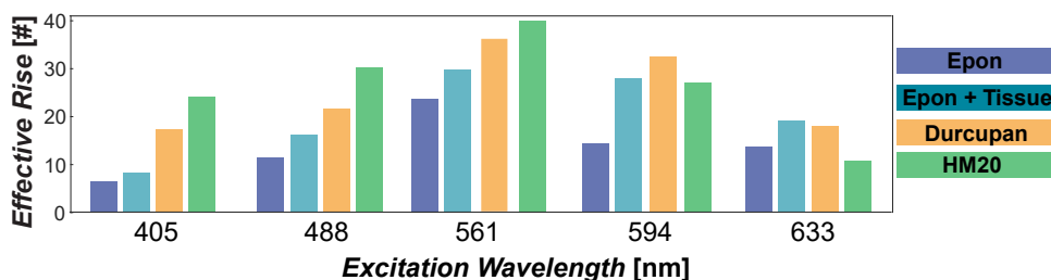
Figure 3.3: Electron beam-induced fluorescence on top of resin auto-fluorescence. Effective rise in electron beam-induced luminescence relative to native auto-fluorescence at the respective excitation wavelengths. The rise in electron-induced signal is strongest at 561nm.
