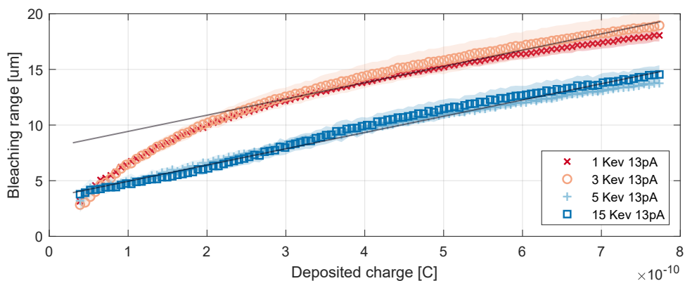
Figure 5.4: Bleaching range as a function of deposited charge for different electron landing energies. The bleaching range increases with the deposited charge. There is a clear distinction in energy levels between where the beam penetrates the perylene layer (5 and 15keV) to reach the conductive ITO coating and where it stops earlier (1 and 3keV). The two parallel straight lines are provided as guides to assist the eye.
