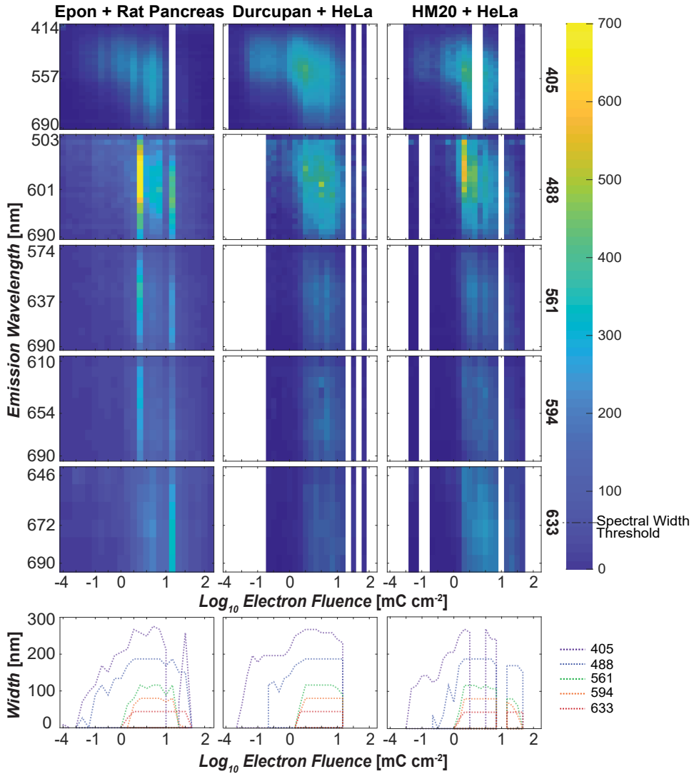
Figure 3.10: Electron-induced luminescence spectrum shows a redshifting pattern with increasing electron fluence, also for bio-embedded resins. (a) Luminescence emission intensity as a function of electron fluence for each of the different excitation wavelengths for Epon + rat pancreas, Durcupan + HeLa cells, and HM20 + HeLa cells. The excitation wavelengths are indicated on the right vertical axis as 405nm, 488nm, 561nm, 594nm, and 633nm, respectively. The color scale denotes intensity according to the indicated scale. Missing pixels are indicated in white. (b) Spectral width as a function of electron fluence for the respective resins in each column at varied excitation wavelengths. The intensity threshold for calculating spectral width is indicated on the color bar. Spectral behavior is similar to the results for bare resins in Figure 3.5.
