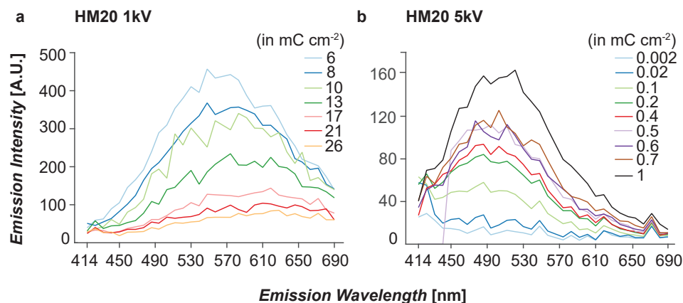
Figure 3.8: Comparison of electron-induced luminescence in methacrylic HM20 with literature results on PMMA [11]. Induced luminescence as a function of emission wavelength for (a) 80nm thick HM20 after irradiation with 1 keV electrons, (b) with 5 keV electrons, both at 405nm excitation. Data in (a) and PMMA [11] cover a similar range in applied electron fluence, but HM20 shows decreasing, redshifting luminescence while PMMA shows increasing, non-shifting induced luminescence. For HM20, the interaction volume is entirely deposited in the sample, while for PMMA, most scattering occurs in the underlying substrate. For HM20 at 5 keV exposure, fluences give a rough approximation of a similar dose deposited in the sample compared to PMMA. HM20 shows a luminescence increase in this range that could also be approximated as spectrally non-shifting. Legends denote respective fluences in \text{mC cm}^{-2} .
