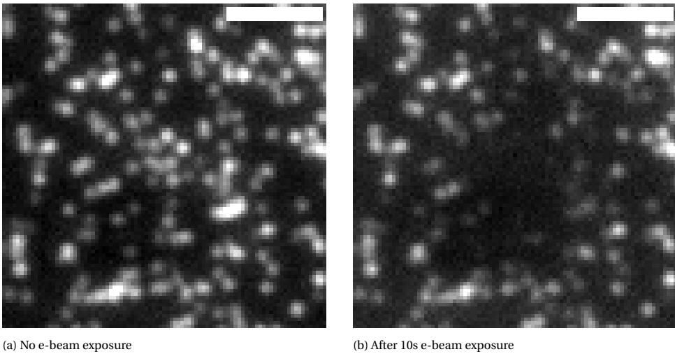
Figure 5.13: FM images of polystyrene microspheres, (a) before and (b) after 10s irradiation with a 1keV landing energy and 13pA current electron beam. Scalebar 3 \mu\text{m} .
