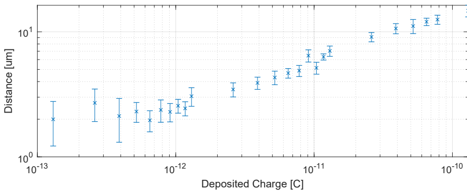
Figure 5.14: Bleaching range as a function of deposited charge measured in a sample of fluorescent polystyrene microspheres spin-coated on an ITO-glass coverslip. The electron beam parameters were set at 1keV landing energy and 13pA current.
