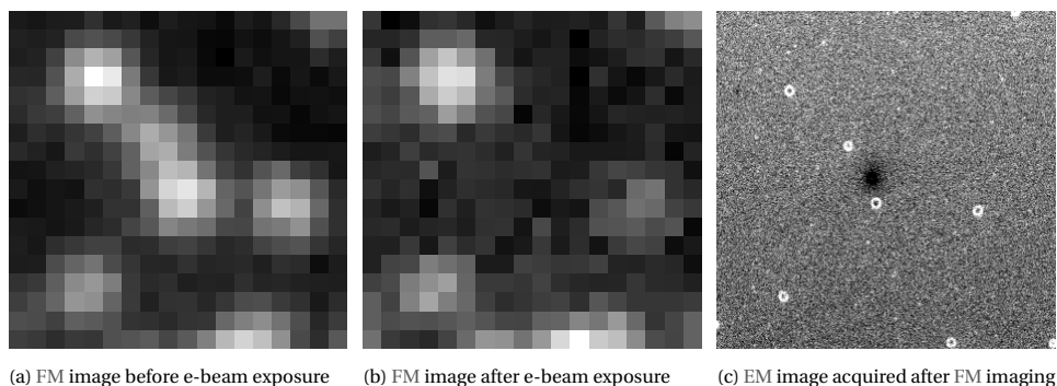
Figure 5.1: Electron-induced fluorescence bleaching extends hundreds of nanometers from stationary electron beam impingement. Panels (a) and (b) show FM images acquired before and after a stationary electron beam was parked in the FOV center for 700ms. Panel (c) shows an EM image acquired immediately after FM imaging, confirming that the beam was in focus. The electron beam parameters were 1keV landing energy and 13pA current. The horizontal field width in each image panel is approximately 2 \mu m.
