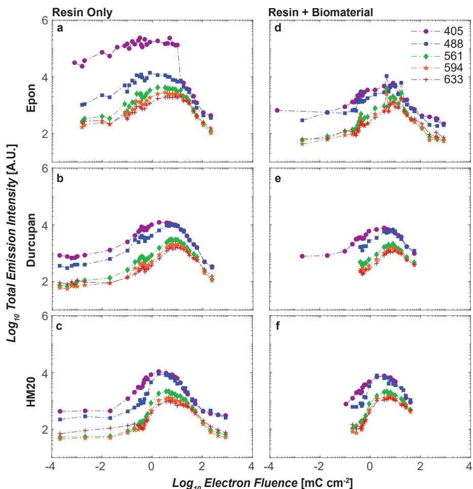
Figure 3.2: Electron-induced luminescence increases, redshifts, and bleaches with increasing electron fluence. Total electron beam-induced luminescence emission intensity as a function of fluence. Colors indicate excitation wavelengths as indicated. (a-c) bare resins and (d-f) samples with embedded biomaterial, namely rat pancreas tissue (d) or HeLa cells (e,f). All data was recorded with 1 keV electron landing energy. Note that bare Epon already shows high UV-excited auto-fluorescence before electron irradiation. Electron-induced luminescence occurs for all resins, with an intensity increase followed by decay.
