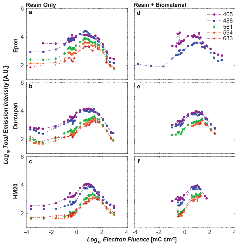
Figure 3.11: Total electron-induced luminescence emission intensity as a function of fluence for each excitation wavelength (shown in color with varied markers) for 5 keV electron landing energy. (a) – (c) and (d) – (f) represent the bare and bio variants respectively. Graphs are displayed in logarithmic scale. The higher landing energy compared to the data in Figure 3.2 (1 keV) results in lowered scattering in the material. The luminescence profiles hence shift to higher fluences.
