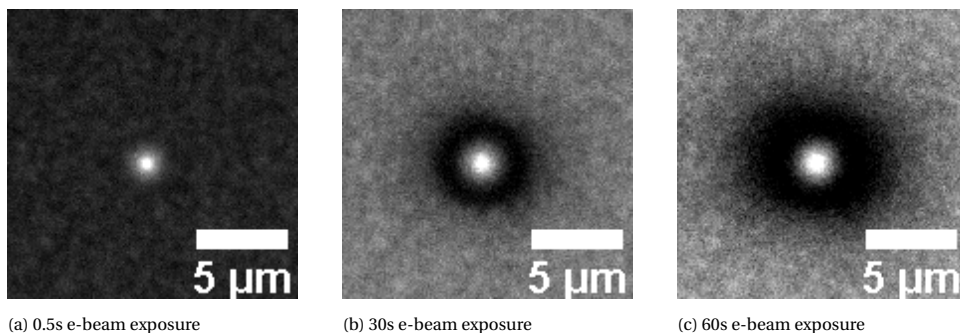
Figure 5.5: FM images of electron-induced bleaching in a bulk fluorescent perylene diimide layer, showing a bright central CL spot. Electron beam parameters are 15keV landing energy and 13pA current. Note that the CL spot is much smaller than the bleached region, indicating that the bleaching is not caused by charge-induced beam defocus. The contrast is adjusted to reduce CL signal clipping.
