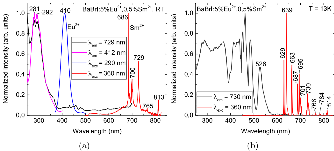
Fig. 3. Emission and excitation spectra of BaBr1:5%Eu 2+ ,0.5%Sm 2+ measured with a Horiba Scientific QuantaMaster fluorometer a) at room temperature and b) with a Newport 66921 xenon lamp in combination with a Horiba Gemini 180 and a Princeton Instruments Acton SP 2300 excitation and emission monochromators, and detected with a Hamamatsu R7600U-20 PMT at 13 K. Emission spectra in a) are corrected for the monochromator and detector efficiencies.
