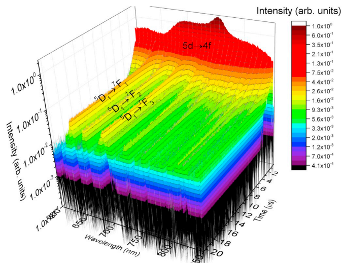
Fig. 9. Time resolved photoluminescence of BaBrI:5%Eu 2+ ,0.5%Sm 2+ at 11 K excited at 360 nm with an OPO laser. The spectrum is not corrected for the monochromator and detector efficiencies.
