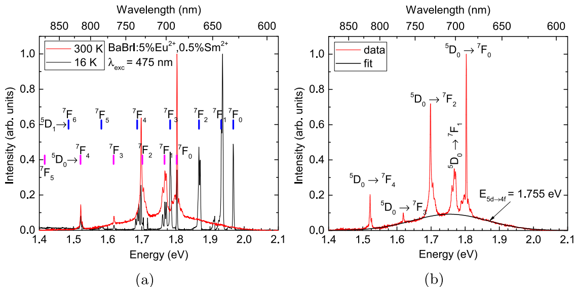
Fig. 4. a.) Emission spectrum of BaBr1:5%Eu 2+ ,0.5%Sm 2+ excited at 475 nm with an OPO laser at 16 K and 300 K. Vertical lines show 4f-4f transition energies of Sm 2+ ion in BaClF measured by Kiss and Weakliem [20] b.) Gaussian fit of the Sm 2+ 5d → 4f emission peak under the 4f → 4f lines observed at 300 K. The spectra are not corrected for the monochromator and detector efficiencies.
