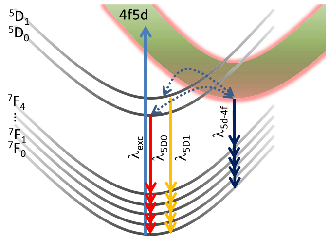
Fig. 12. Configurational coordinate diagram of \text{Sm}^{2+} in BaBrI. Solid arrows indicate radiative, dotted arrows non-radiative processes.
