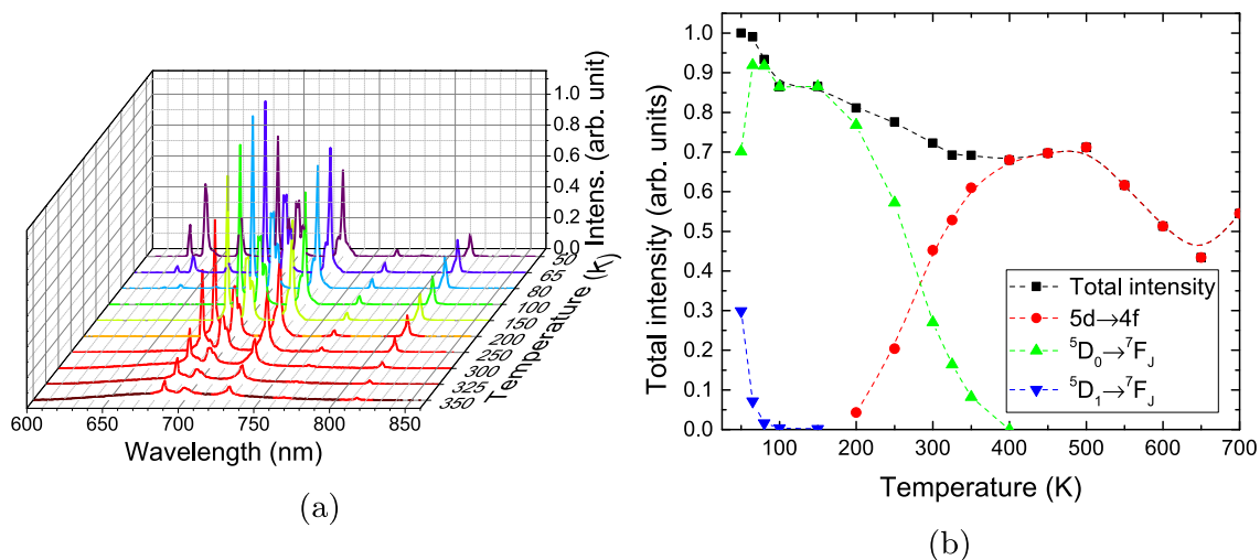
Fig. 11. a.) Photoluminescence emission spectrum of \text{Sm}^{2+} in BaBrI:5% \text{Eu}^{2+} , 0.5% \text{Sm}^{2+} versus temperature using 360 nm photoluminescence excitation b.) Intensity of different \text{Sm}^{2+} transitions in BaBrI:5% \text{Eu}^{2+} , 0.5% \text{Sm}^{2+} versus temperature using 360 nm photoluminescence excitation.
