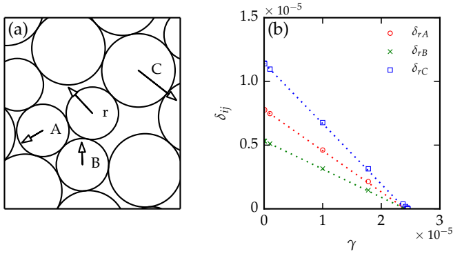
FIG. 2. (a) Zoom-in of a packing where particle r becomes a rattler after the first contact change ( N = 22 , P = 1.5 \times 10^{-5} ). Neighboring particles A , B , and C are indicated. (b) Overlap of r with the neighboring particles A , B , and C as a function of strain \gamma . Markers are direct numerical simulation (DNS) data points, lines indicate the linear response prediction. The DNS and LR predictions for rattler creation are \gamma_*^{\text{DNS}} = 2.45 \times 10^{-5} and \gamma_*^{\text{LR}} = 2.41 \times 10^{-5} .
