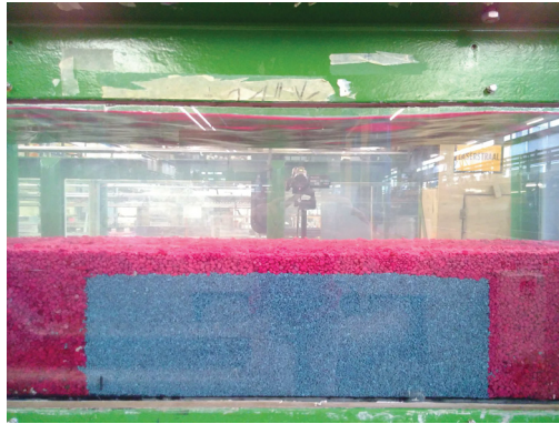
Figure 1. Initial condition of the experimental set-up. A patch of fine sediment (blue) is embedded in coarse sediment (red).
