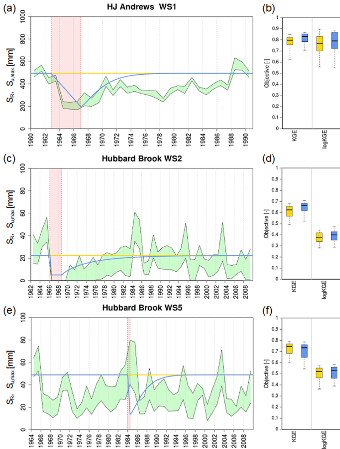
Figure 8. The time invariant S_{u,max} formulation represented by S_{R,20yr} (yellow) and time dynamic S_{u,max} fitted Weibull growth function (blue) with a linear reduction during deforestation (red shaded area) and mean 20-year return period root-zone storage capacity S_{R, 20yr} as equilibrium value for (a) HJ Andrews WS1 with a = 0.0001 \text{ days}^{-1} , b = 1.3 and S_{R,20yr} = 494 \text{ mm} with (b) the objective function values, (c) Hubbard Brook WS2 with a = 0.001 \text{ days}^{-1} , b = 0.9 and S_{R,20yr} = 22 \text{ mm} with (d) the objective function values, and (e) Hubbard Brook WS5 with a = 0.001 \text{ days}^{-1} , b = 0.9 and S_{R,20yr} = 49 \text{ mm} and with (f) the objective function values. The green shaded area represents the maximum and minimum boundaries of S_{R,1yr} from the water balance-based estimation, caused by the sampling of interception capacities.
