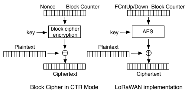
Fig. 2. LoRaWAN uses a AES in counter mode for message encryption.
