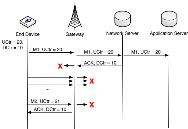
Fig. 11. ACK messages may be repurposed to acknowledge other frames than originally received by the application provider.
