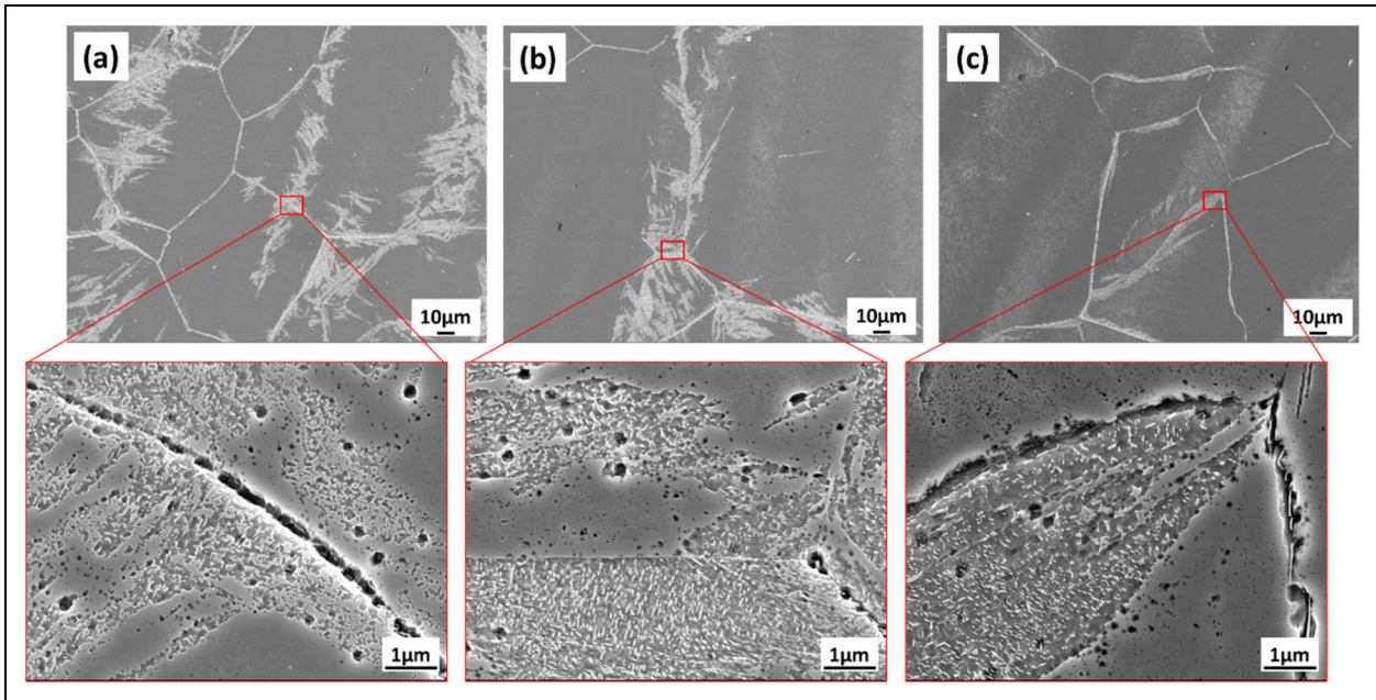
Figure 10. SEM images of HMn Q&P specimen with decreasing volume fraction of MI: (a) specimen quenched to 75°C, (b) specimen quenched to 100°C, (c) specimen quenched to 125°C.
