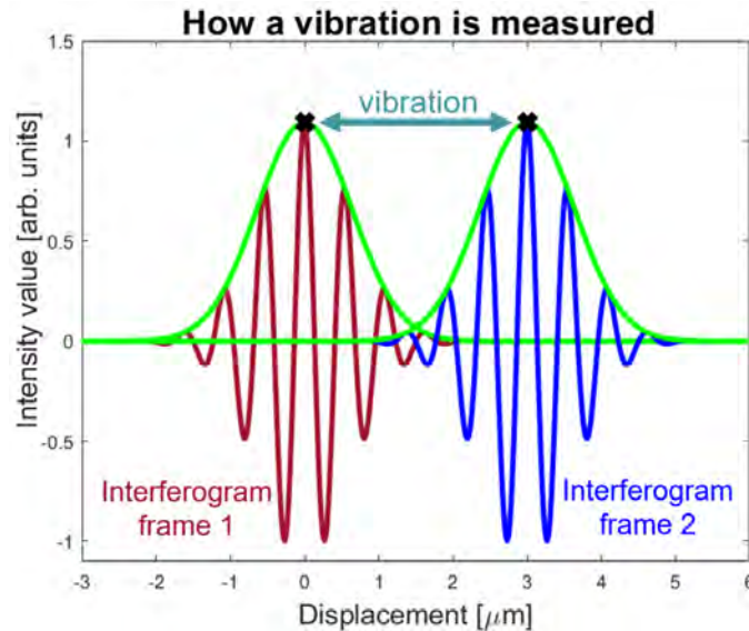
Figure 2. Illustration of the second application of the metrology instrument we developed, detecting local induced vibrations. We measure a local induced vibration as the displacement of the peak of the coherence envelope of the local interferogram at two consecutive camera frames. The temporal resolution of the measurements depends on the frame rate of the camera used
