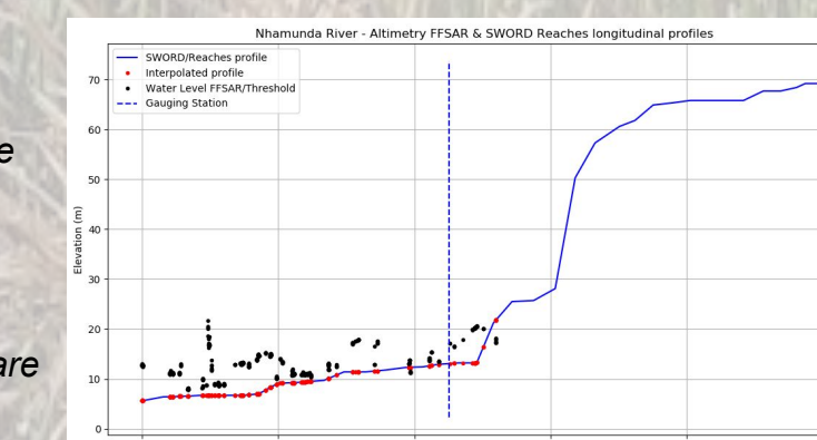
Figure 2: (Black dots) FF-SAR/Threshold retracker along the longitudinal path of the river. (Blue curve) Mean river profile derived from the SWORD data base and (vertical dashed line) the location of the ANA gauging station.
