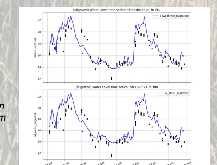
Figure 3: (Black) L2 river water level time series, (blue) gauging data.
