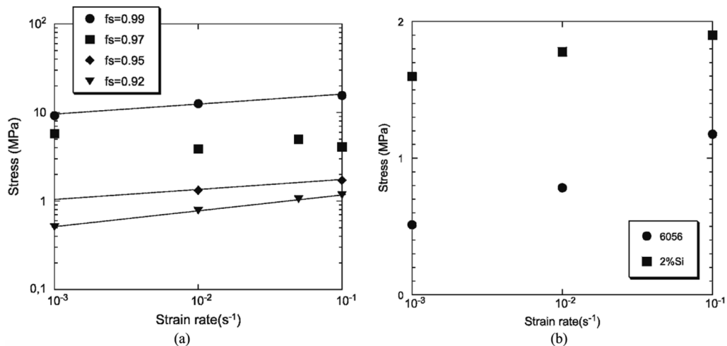
Fig. 3.21. (a) Maximum stress (i.e., UTS) versus strain rate at different solid fractions ( f_s ) for AA6056 alloys upon reheating, (b) maximum stress versus strain rate at the solid fraction of 0.9 for AA6056 alloys and the alloys with 2 wt% Si [41].
