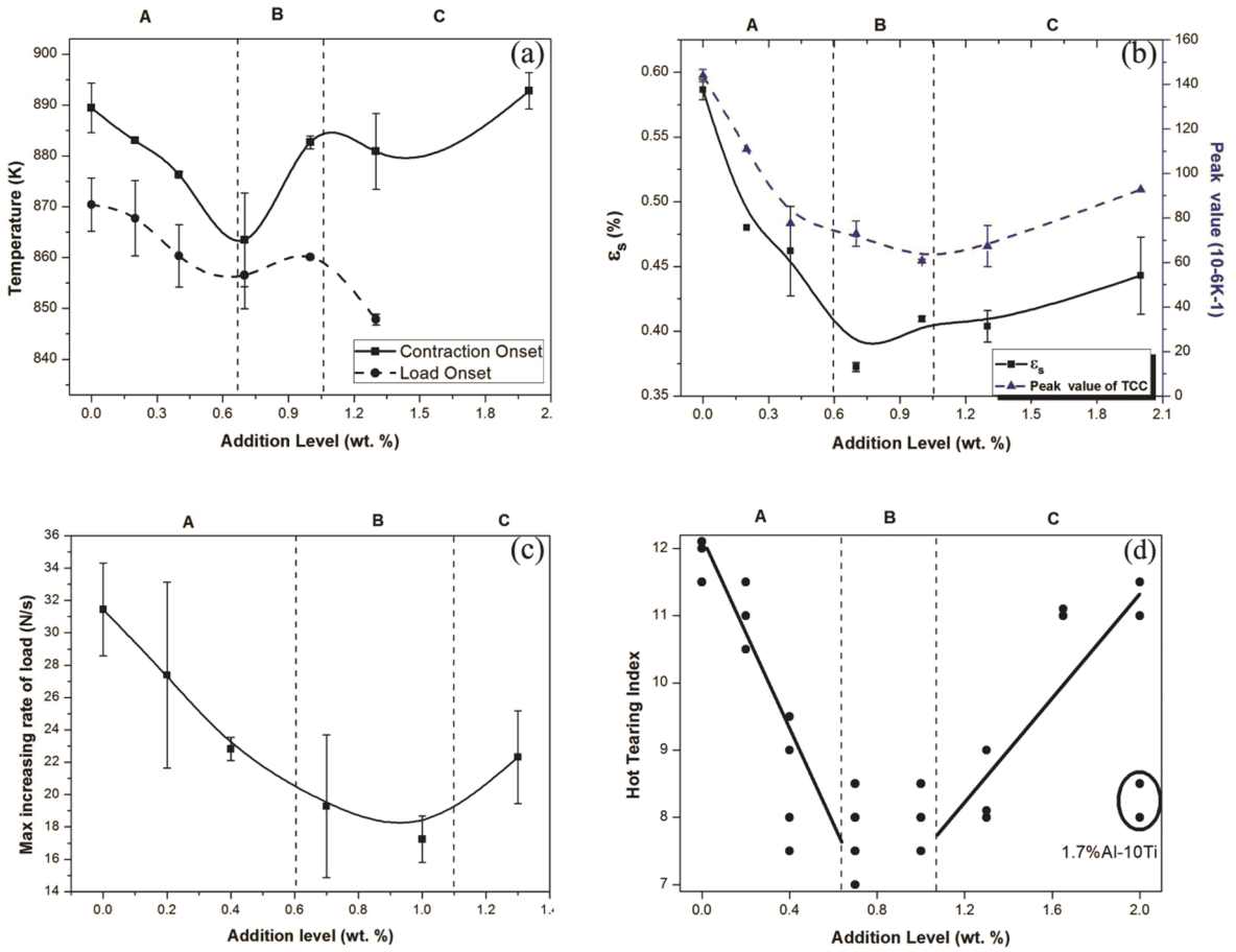
Fig. 3.10. Effect of the addition of Al-5Ti-1B on the contraction, load behaviour, and hot tearing susceptibility of AA7050 alloy: (a) the temperature corresponding to the contraction and load onset; (b) the linear contraction ( \epsilon_s ) and the peak value of the TCC; (c) the maximum increasing rate of load; (d) the hot tearing susceptibility [26].
