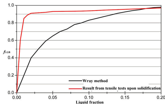
Fig. 5.1. Fraction of grain boundary area covered by liquid phases ( f_{LGB} ) from Wray method and tensile tests under solidification [111].
