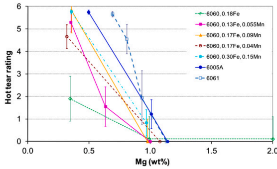
Fig. 4.4. Variance of hot tearing susceptibility with Mg content in various AA6xxx alloys [65].
