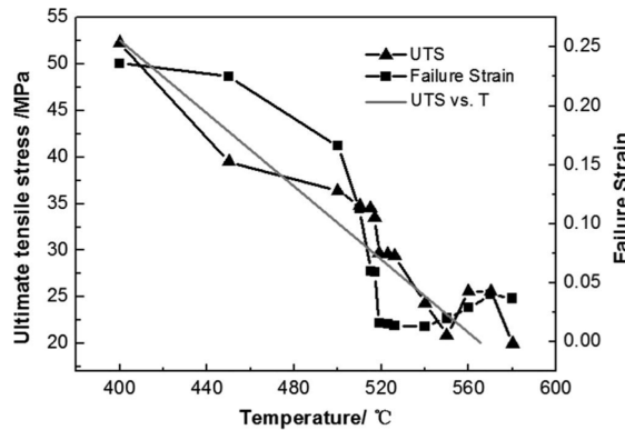
Fig. 3.33. Variations of UTS and failure strain with temperature for extruded AA7075 alloy [37]. The tests were performed upon reheating.
