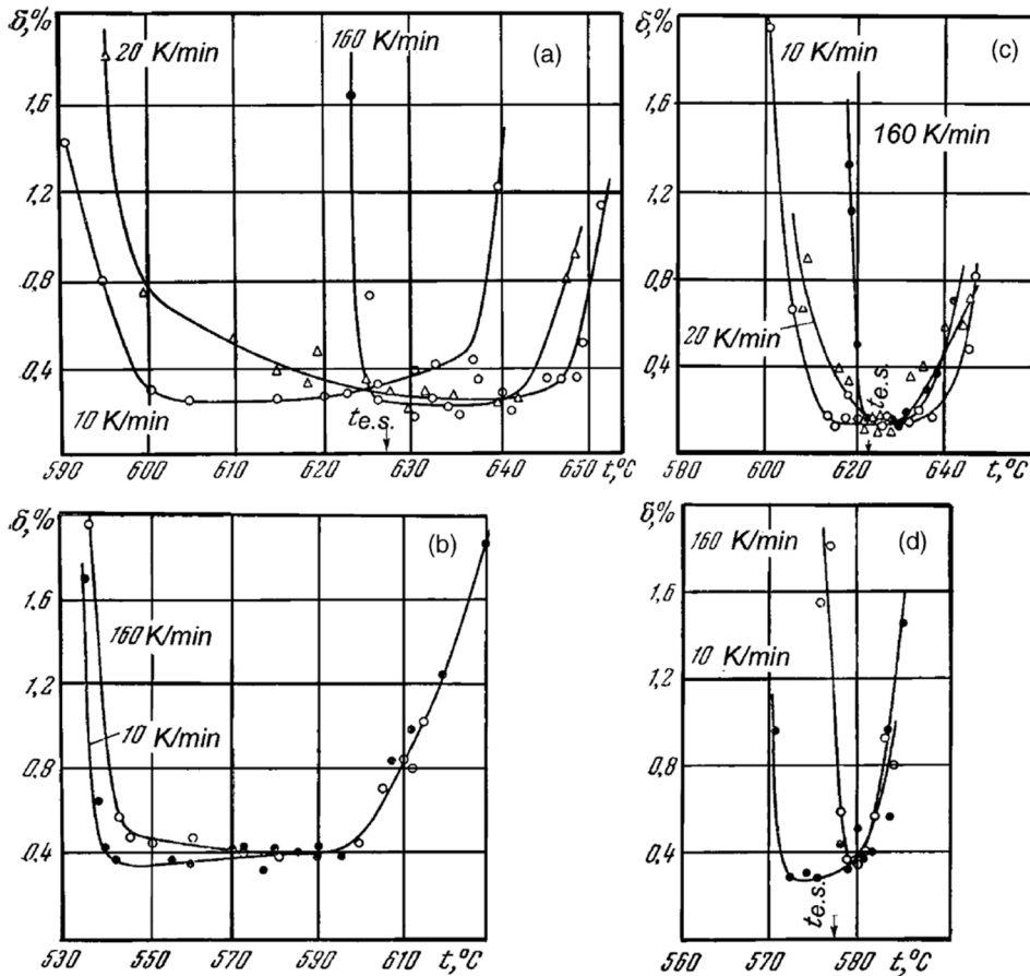
Fig. 3.20. Effect of cooling rate on the semi-solid elongation ( \delta ) of (a) Al-1.5 wt% Cu, (b) Al-5 wt% Cu, (c) Al-0.7 wt% Si, and (d) Al-5 wt% Si. t_{e.s.} is the equilibrium solidus, and the NES is 548 and 577 °C for Al-Cu and Al-Si alloys, respectively [15]. The testing method is the same as that used in Fig. 3.18.
