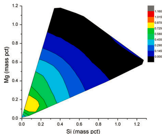
Fig. 4.3. Hot tearing susceptibility of refined Al-Mg-Si alloys [64].
