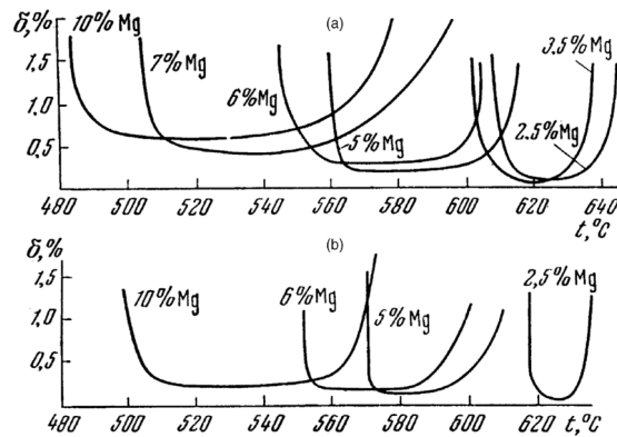
Fig. 3.28. Variance of semi-solid elongation ( \delta ) with temperature in (a) as-cast and (b) deformed Al–Mg alloys [15]. The testing method is the same as that used in Fig. 3.18.
