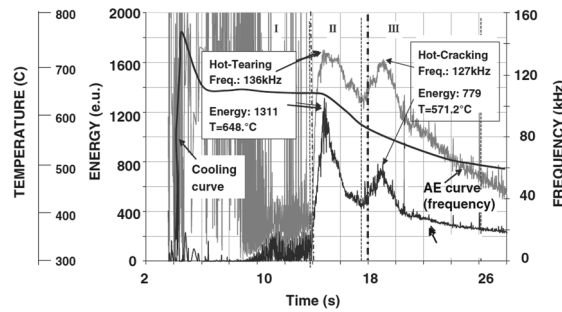
Fig. 2.14. AE average frequency and energy vs time plotted with the cooling curve [48].
