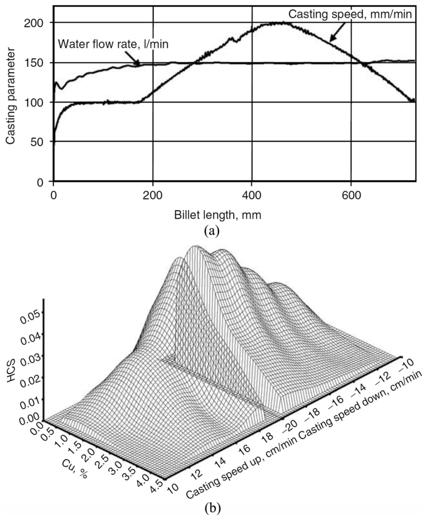
Fig. 4.1. (a) Experimental scheme of DC casting with ramping up and down the casting speed, (b) effect of Cu content and casting speed on the measured hot tearing susceptibility in Al-Cu alloys during DC casting [110].
