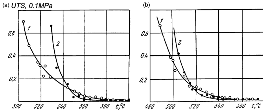
Fig. 3.27. Variation of UTS with the temperature of (1) as-cast and (2) hot-rolled and homogenized alloys: (a) Al–7 wt% Mg and (b) Al–10 wt% Mg [15]. The testing method is the same as that used in Fig. 3.18.
