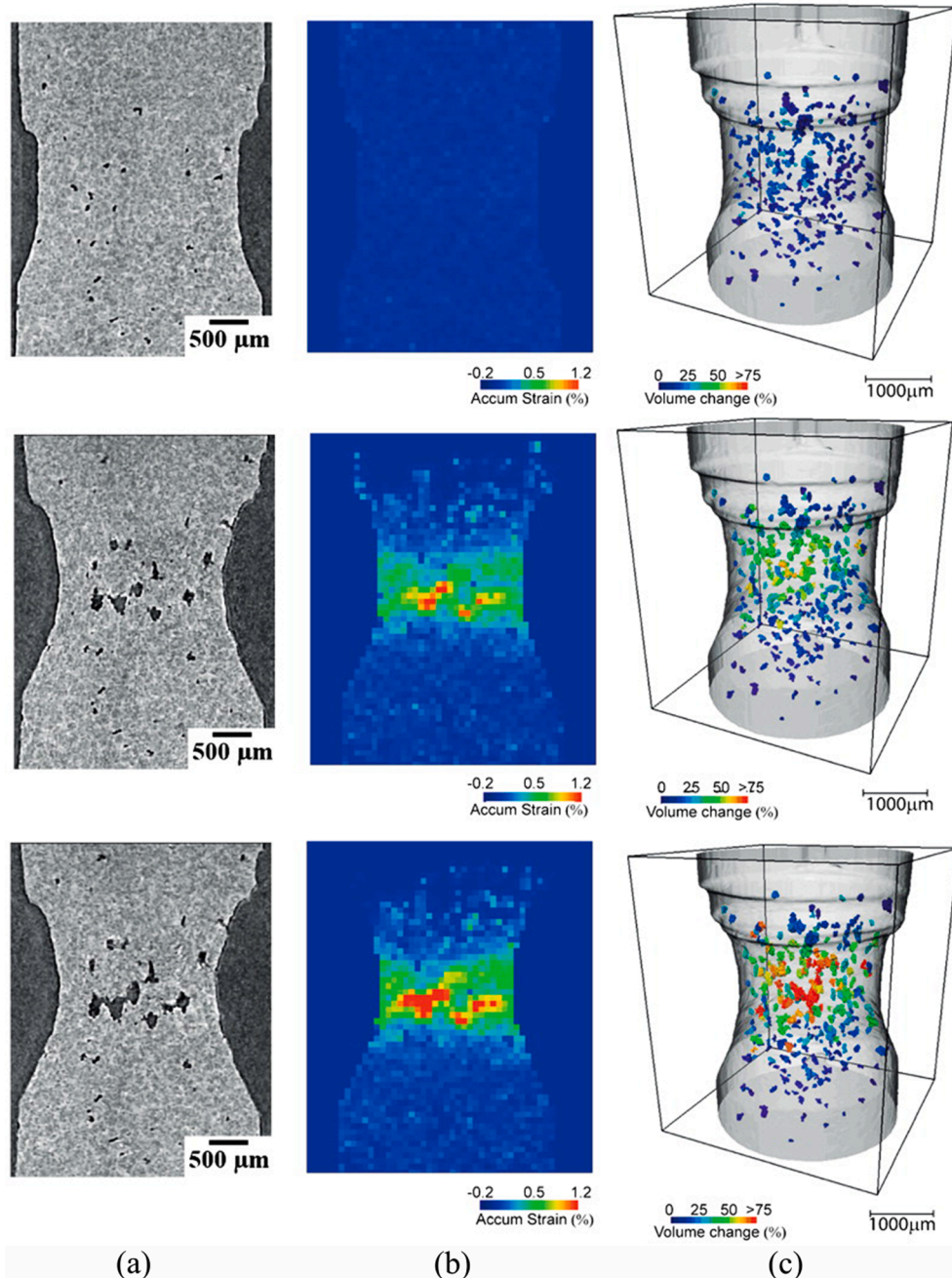
Fig. 2.11. 3D images obtained by semi-solid tensile testing in an Al-Cu alloy: (a) longitudinal sections of typical 3D damage evolutions during the hot tearing, (b) the local strain field measured by digital volume correlation between continuous photos, and (c) the variation of void volume corresponding to the original volume at the initial stage of hot tearing [86].
