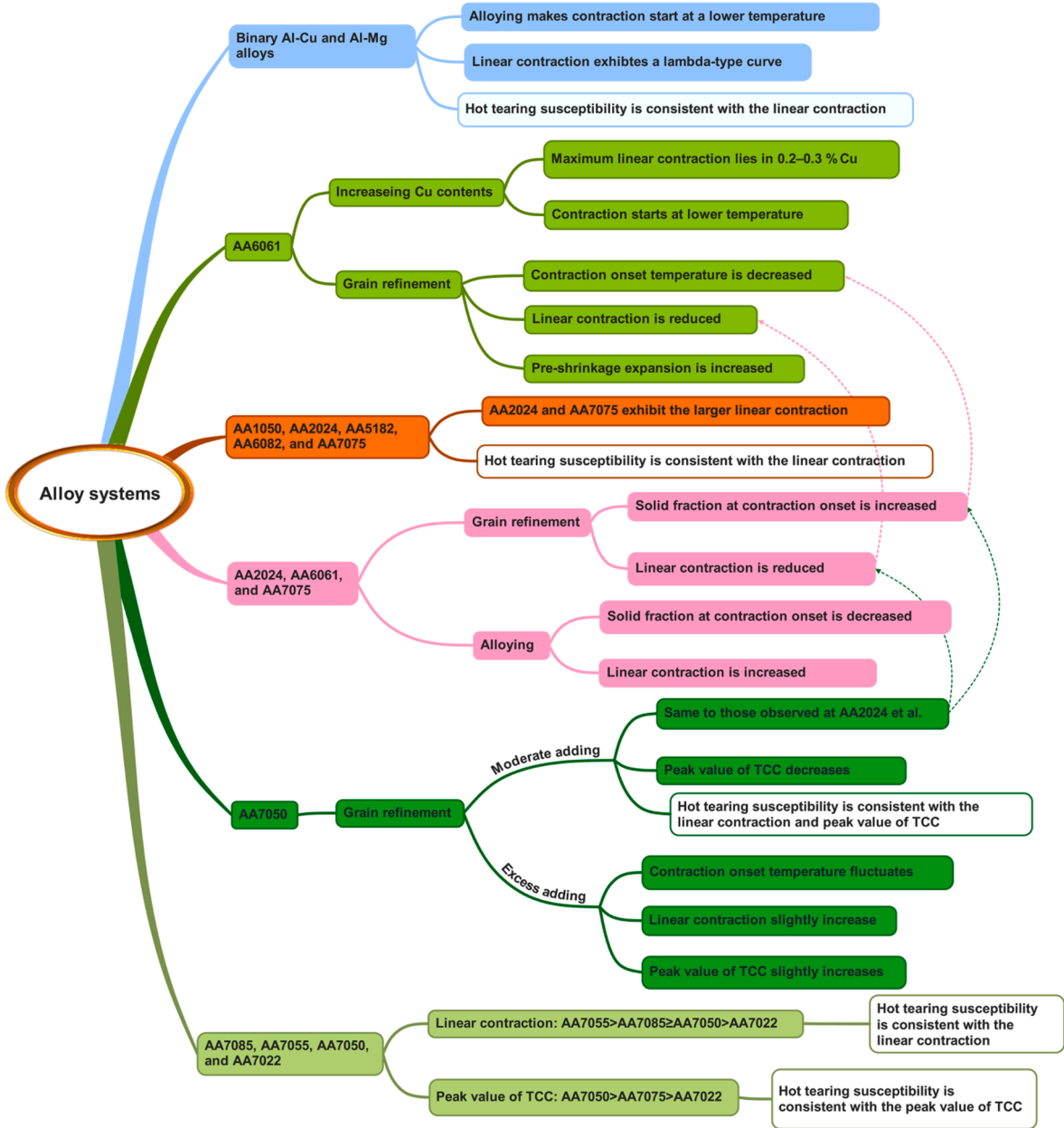
Fig. 3.6. An outline of the linear contraction behaviour of some binary and commercial aluminium alloys. Dotted lines mean that there are similarities between the chosen items.
