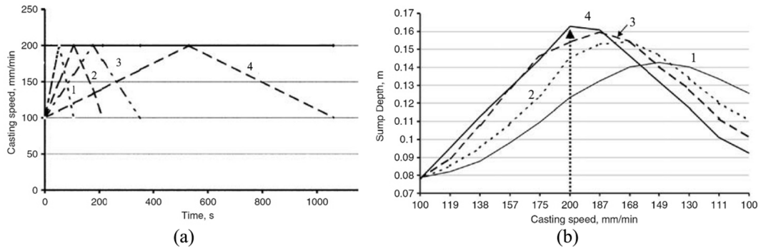
Fig. 5.5. (a) Four kinds of ramping casting modes, (b) effect of different ramping casting rates on the evolutions of the calculated sump depth in a 200-mm Al-4 wt% Cu billet [154].
