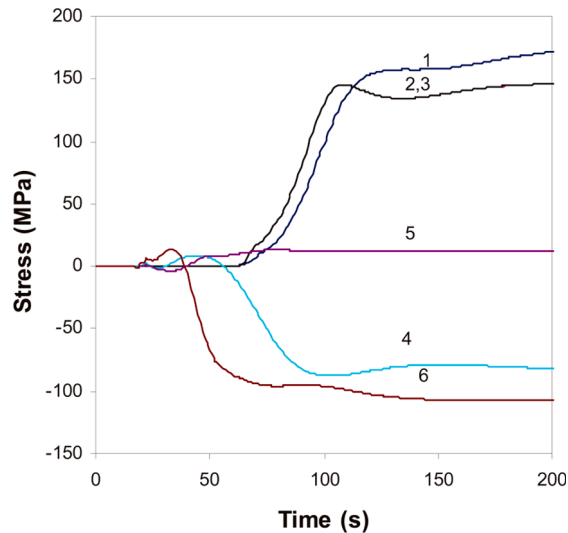
Fig. 5.3. Calculated stresses development during steady-state stage in a DC-casting 200-mm Al-4.5 wt% Cu round billet (casting speed: 120 mm/min): axial (1), radial (2) and circumferential (3) stresses at the centre of the billet, and axial (4), radial (5) and circumferential (6) stresses at the periphery (10 mm from the surface) [143].
