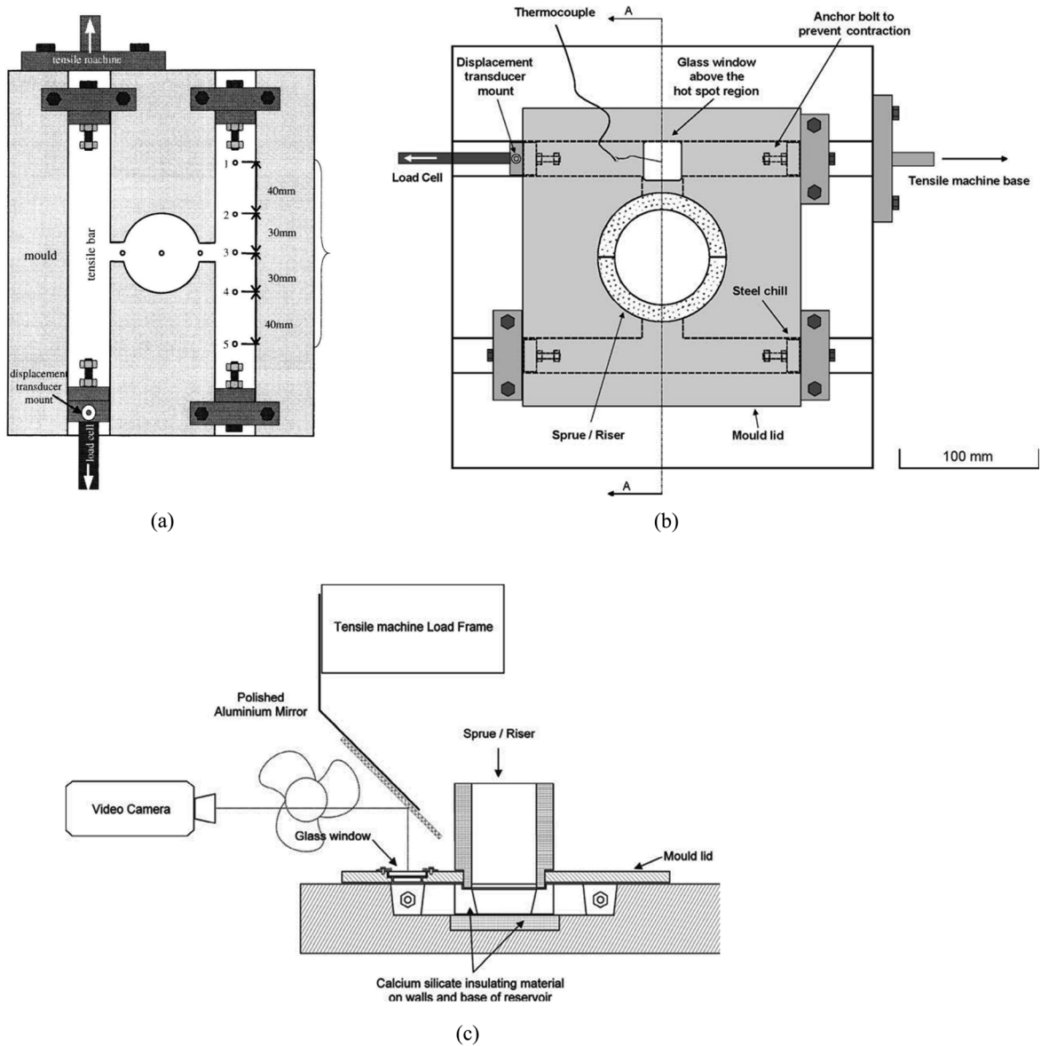
Fig. 2.7. (a) Schematic of the CHT rig developed by Instone et al. [62], (b) improved CHT rig with an observation system, and (c) cross-section of the improved rig through section A-A in (b) [70].
