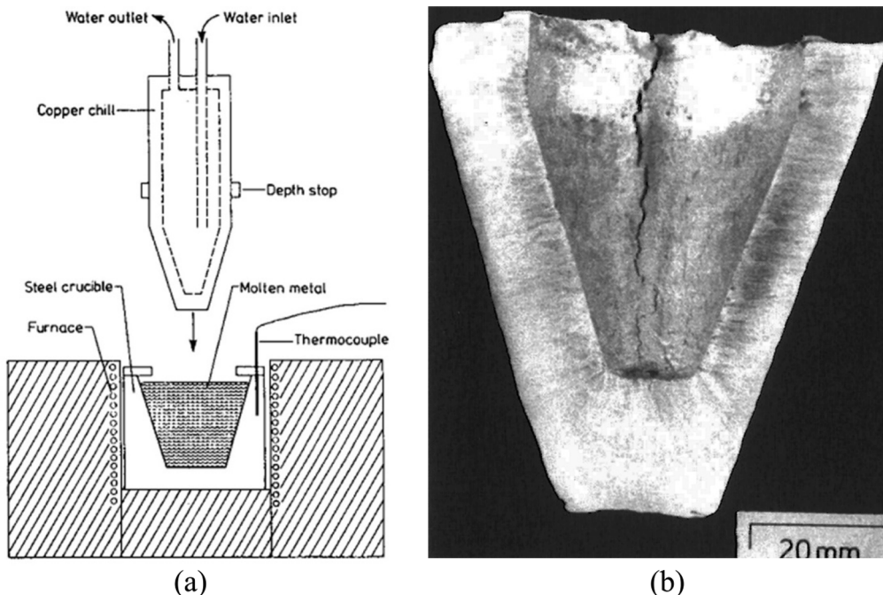
Fig. 2.4. Schematic of a “cold finger” mould and the corresponding casting [56,57].
