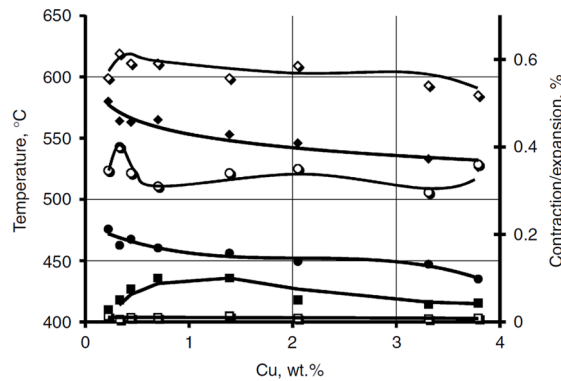
Fig. 3.8. Effect of Cu contents and grain refinement on the expansion/contraction behaviour of 6061-type alloys [14]: \diamond , \blacklozenge = contraction onset temperature; \circ , \bullet = contraction to NES (assuming to be 500 °C), %; and \square , \blacksquare = pre-shrinkage expansion. Open symbols correspond to non-grain-refined alloys and solid symbols correspond to grain-refined alloys.
