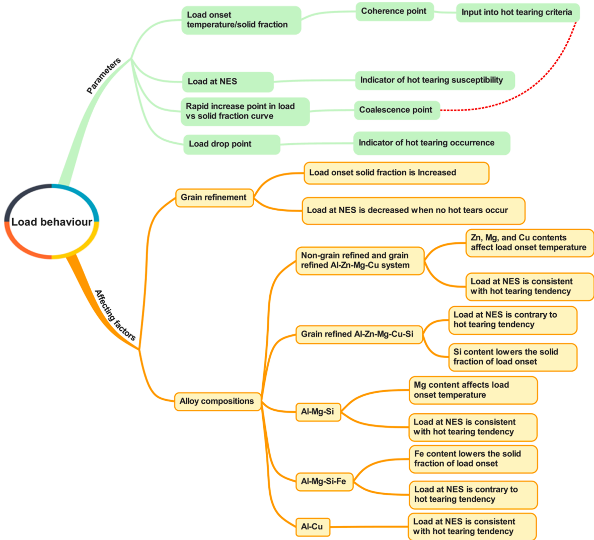
Fig. 3.13. An outline of the load behaviour during solidification, including the quantitative data obtained from the load curve during solidification and influence factors on the load behaviour.
