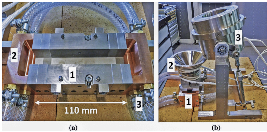
Fig. 2.6. (a) Dog-bone-shaped mould: 1, steel mould; 2, water-cooled copper mould; and 3, water pipe; (b) experimental device including 1, dog-bone-shaped mould; 2, feeder; and 3, rotating pouring system [58].
