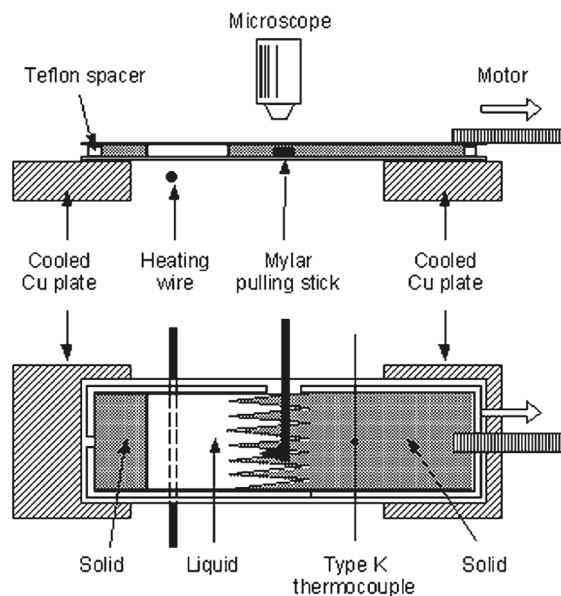
Fig. 2.9. Schematic of the experimental setup used by Farup et al. [80].
