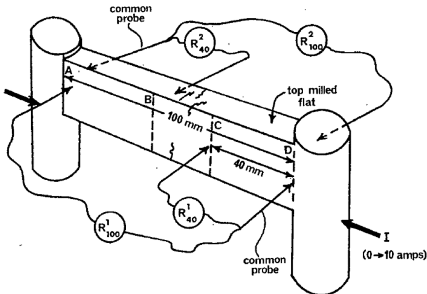
Fig. 2.13. The setup of the measurement of electrical resistance [60].
