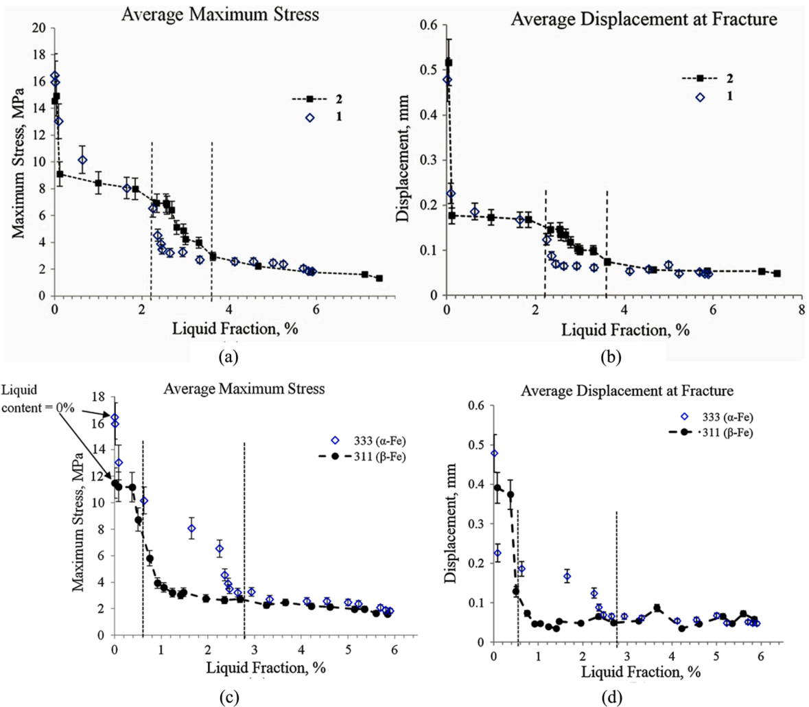
Fig. 3.17. (a) Maximum stress (i.e., UTS) and (b) displacement at fracture of Al-Cu 206 cast alloys containing 0.3 wt% Si and 0.3 wt% Mn (“Alloy 333”) versus liquid fraction (1, no refiners; 2, adding 0.4 wt% Al-5Ti-1B alloys); comparison of (c) maximum stress and (d) displacement at fracture of “Alloy 333” and “Alloys 311” (Al-Cu 206 cast alloys containing 0.1 wt% Si and 0.1 wt% Mn) versus liquid fraction [36]. The tests were performed upon reheating.
