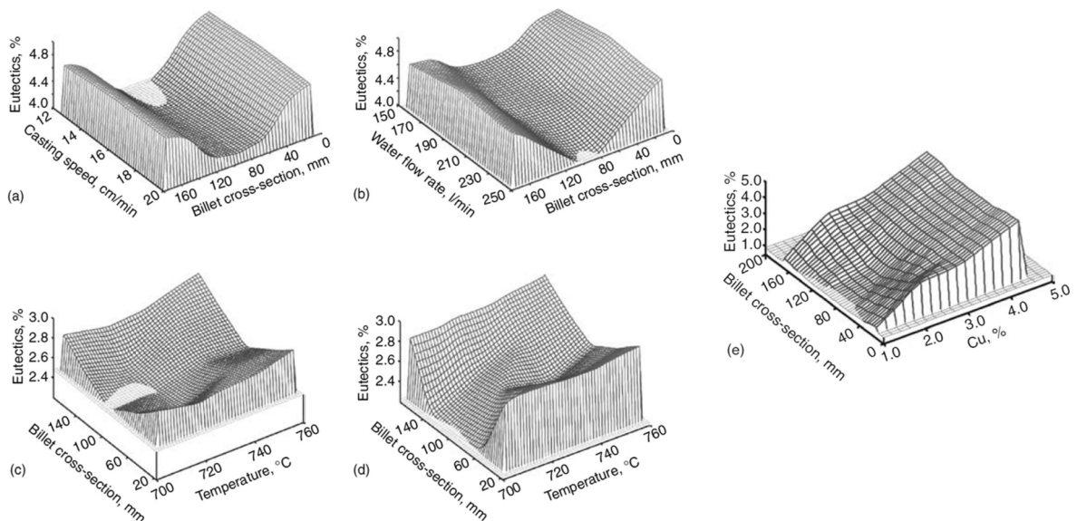
Fig. 4.8. Effect of compositions and process parameters on the amount and distribution of measured non-equilibrium eutectics in the Al-Cu system: (a) Al-4.3 wt% Cu, water flow rate 150 l/min, melt temperature 715 °C; (b) Al-4.3 wt% Cu, casting speed 200 mm/min, melt temperature 715 °C; (c) Al-2.8 wt% Cu, water flow rate 150 l/min, casting speed 100 mm/min; (d) Al-2.8 wt% Cu, water flow rate 150 l/min, casting speed 200 mm/min; (e) water flow rate 150 l/min, casting speed 200 mm/min [7,110,133].
