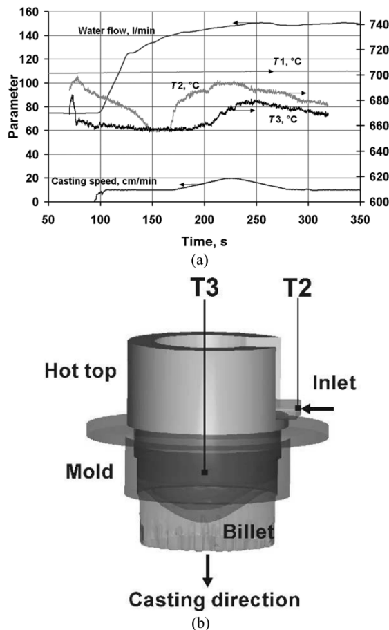
Fig. 4.10. Casting setup and the positions of thermocouples [133].
