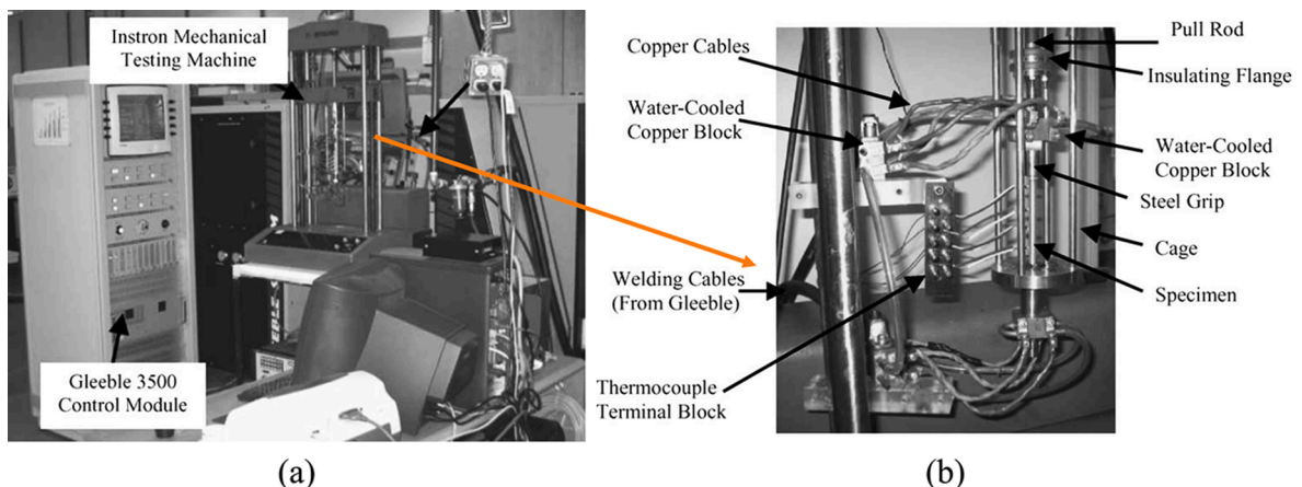
Fig. 2.2. (a) Example of a Gleeble 3500 thermo-mechanical testing machine for semi-solid tensile tests; (b) details of the tensile unit [42].
