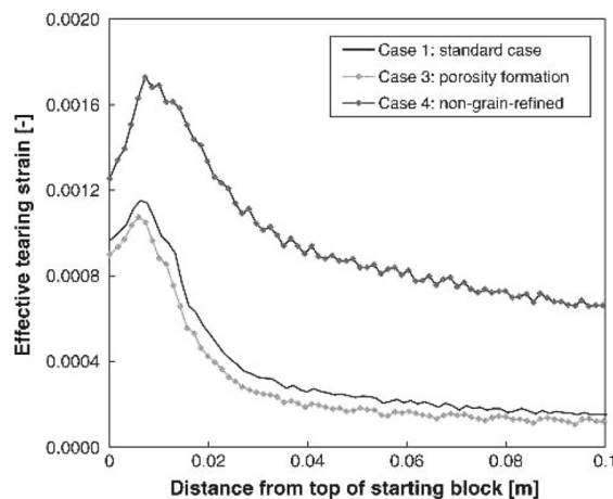
Fig. 5.8. Effective tearing strain for ( w_t = 1 , w_{d=0} ) when viscoplastic deformation is taken into account (Case 1), when pressure relaxation due to microporosity is taken into account (Case 3), and when a non-grain-refined microstructure is considered (Case 4) [150].
