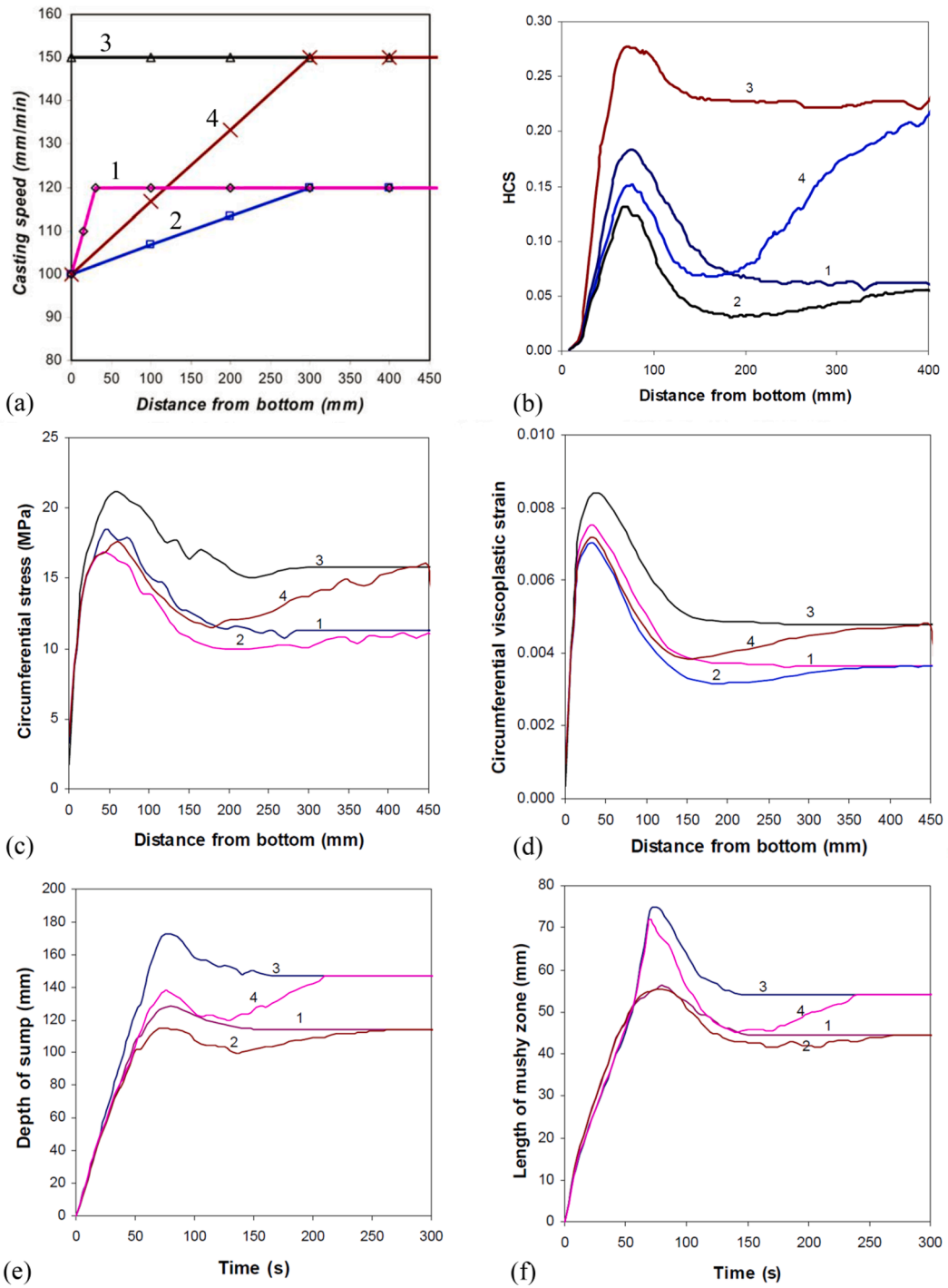
Fig. 5.4. Thermomechanical simulations of a DC-casting 200-mm Al-4.5 wt% Cu alloy billet: (a) case studies on casting-speed ramping in the start-up phase of casting; corresponding developments of (b) predicted HCS, (c) circumferential stress, (d) circumferential strain at solidus temperature, (e) depth of sump, and (f) length of mushy zone in the centre of the billet [143,144].
