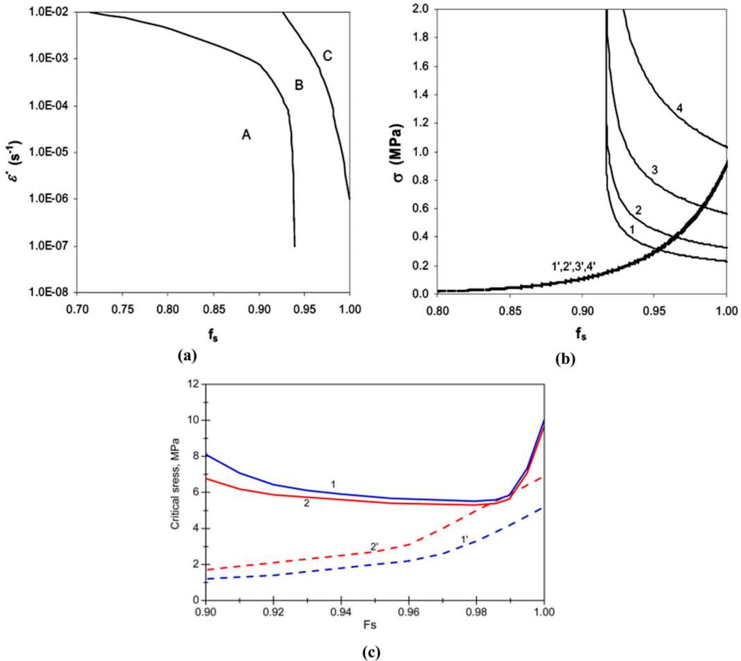
Fig. 5.7. (a) Three regions (A = micro-pores and hot tears are absent, B = micro-pores develop but hot tears do not form, and C = hot tears are formed); (b) effect of grain size on the developed stress in the mush (1'–4') and the critical stress (1–4): 1,1', 600 \mu\text{m} ; 2,2', 300 \mu\text{m} ; 3,3', 100 \mu\text{m} ; and 4,4', 30 \mu\text{m} ; (c) effect of casting speed on the developed stress (dash line) in the mush and the critical stress (solid line): 1,1', 25 mm min -1 and 2,2', 35 mm min -1 [111,144].
