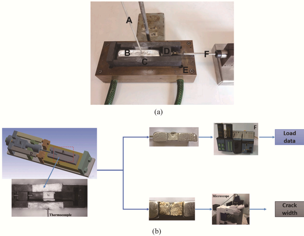
Fig. 2.8. (a) T-shaped displacement testing device developed by Eskin et al. [71] and (b) modified by Li et al. with a load cell [77].
