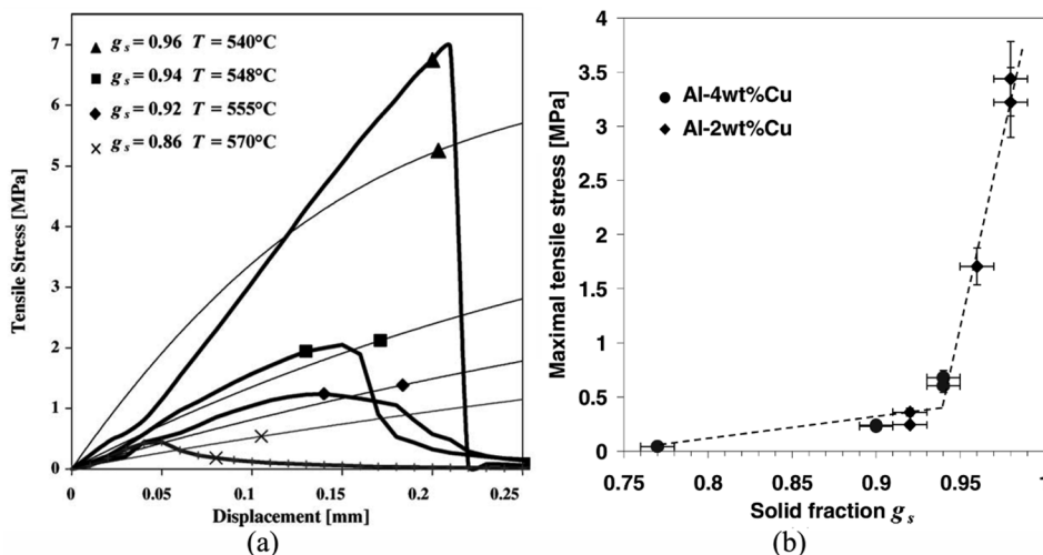
Fig. 3.31. (a) Tensile curves of AA5182 alloy at different temperatures or solid fractions (experimental (thick curves) and predicted results (thin curves)), and (b) variation of UTS with the solid fraction of two Al-Cu alloys [20,21]. The tests were performed upon solidification.
