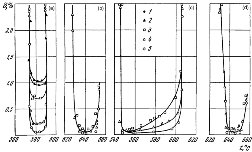
Fig. 3.26. Variance of semi-solid elongation ( \delta ) with temperature during solidification (1, 2) and reheating (3, 4, 5) in different deformation rates (1–4: 2, 5, 8, and 80 mm/min, respectively; 5: dynamic loading) of (a) Al–5 wt% Si, (b) Al–0.6 wt% Si, (c) Al–6.5 wt% Cu, and (d) Al–1.5 wt% Cu [15]. The testing method is the same as that used in Fig. 3.18.
