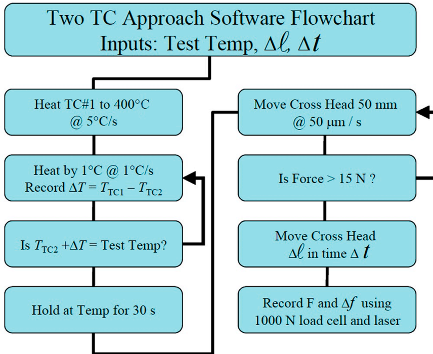
Fig. 2.3. Flowchart outlining the “2TC technique” for performing the semi-solid tensile test in the Gleeble 3500 thermo-mechanical simulator [40].
