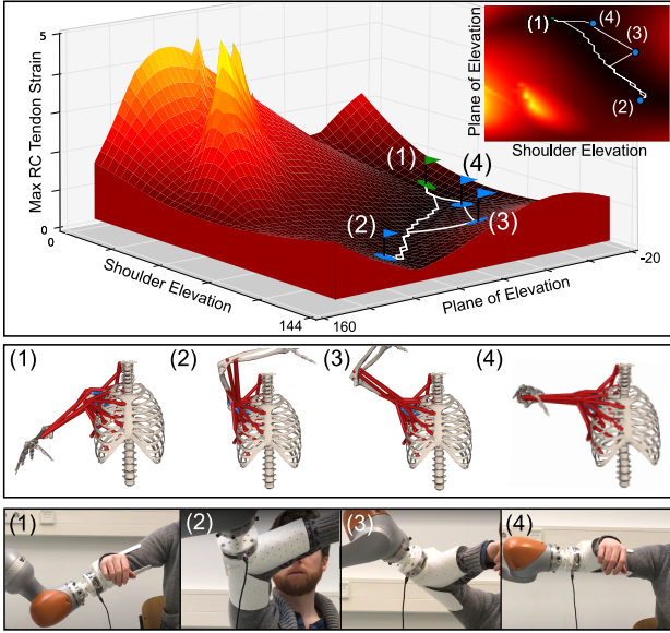
Fig. 5. Example of a low tendon-strain trajectory of the shoulder within the 3D strain map set by a user-specified start point (1) and three waypoints, flags (2), (3), and (4). Inset is a top-down view. Corresponding configurations of the biomechanical model are shown in the middle row and the actual human arm configurations as controlled by the robotic manipulator are captured in the bottom row.
