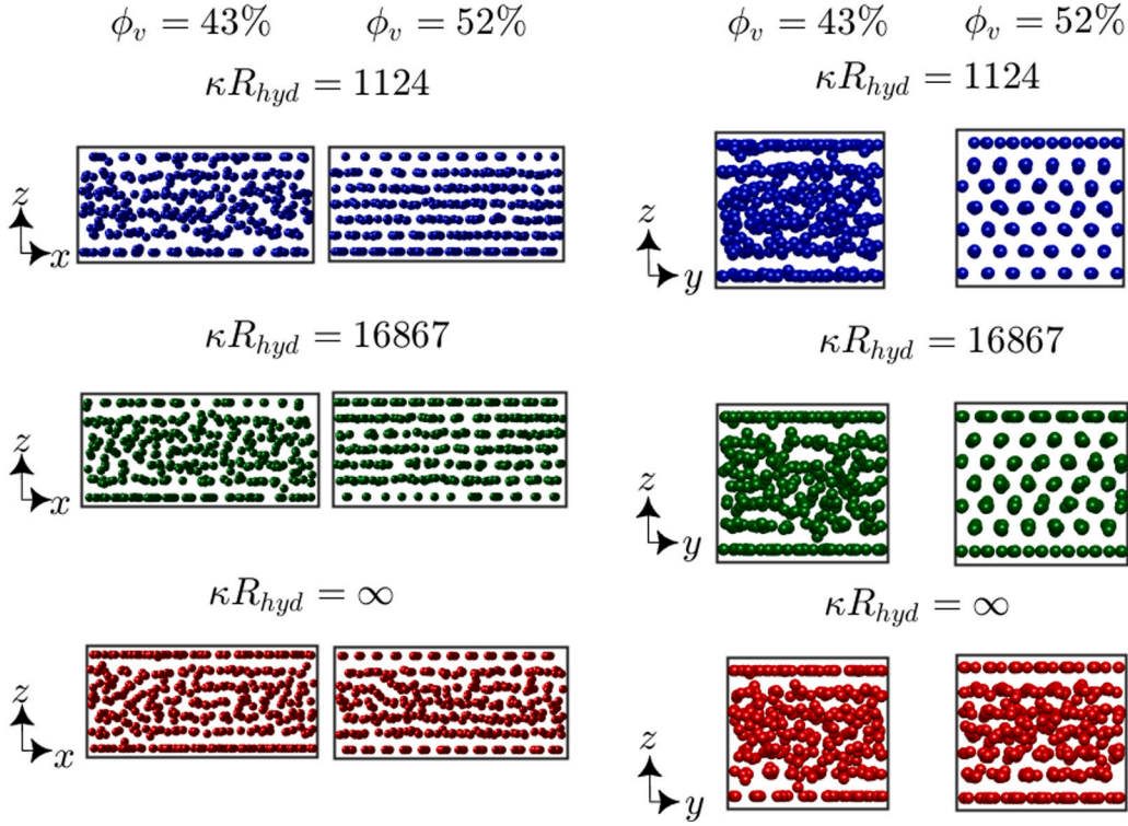
Fig. 8. Left panel: x-z visualisations of particles are shown for \phi_v = 43 and 52%. Right panel: y-z visualisations of suspended particles with 43 and 52% solids are compared. In both panels, from top to bottom, the magnitude of \kappa R_{hyd} increases from 1124 to \infty . The radius of each sphere is drawn half of its original size and the particle Reynolds number Re_p = 0.1 . (For interpretation of the references to colour in this figure legend, the reader is referred to the web version of this article.)
