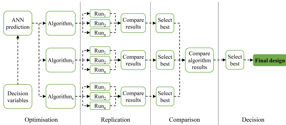
Fig. 5. MUZO optimisation process and decision framework.
