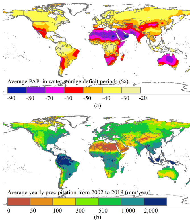
Fig. 6. (a) Average precipitation deficit percentage in water storage deficit periods. (b) GPM-based average yearly precipitation from 2002 to 2019.
