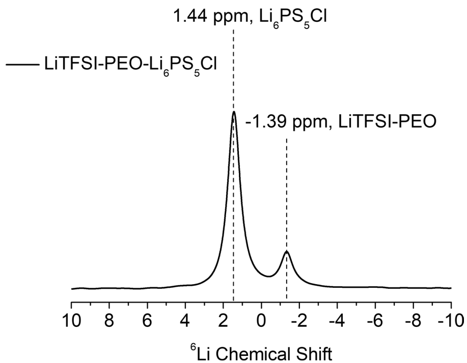
Extended Data Fig. 3 | 1\text{D } {}^6\text{Li} magic angle spinning (MAS) spectrum corresponding to the \text{Li}_6\text{PS}_5\text{Cl} -LiTFSI-PEO HSE. 1\text{D } {}^6\text{Li} magic angle spinning (MAS) spectrum corresponding to the \text{Li}_6\text{PS}_5\text{Cl} -LiTFSI-PEO HSE.
