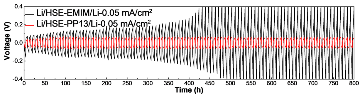
Extended Data Fig. 8 | Plating and stripping curves of a Li metal symmetrical cell with HSE-EMIM and HSE-PP13. Plating and stripping curves of a Li metal symmetrical cell with LiTFSI-PEO-Li 6 PS 4 Cl HSEs with PP13 TFSI and EMIM TFSI ionic liquids. The cell with HSE-EMIM shows quick polarization after 300 h of cycling at a current density of 0.05 mA/cm 2 . In comparison the cell with HSE-PP13 shows a very stable over-potential (lower than 200 mV) during 800 hours of cycling, indicating a higher ionic conductivity and better interfacial stability against Li-metal.
