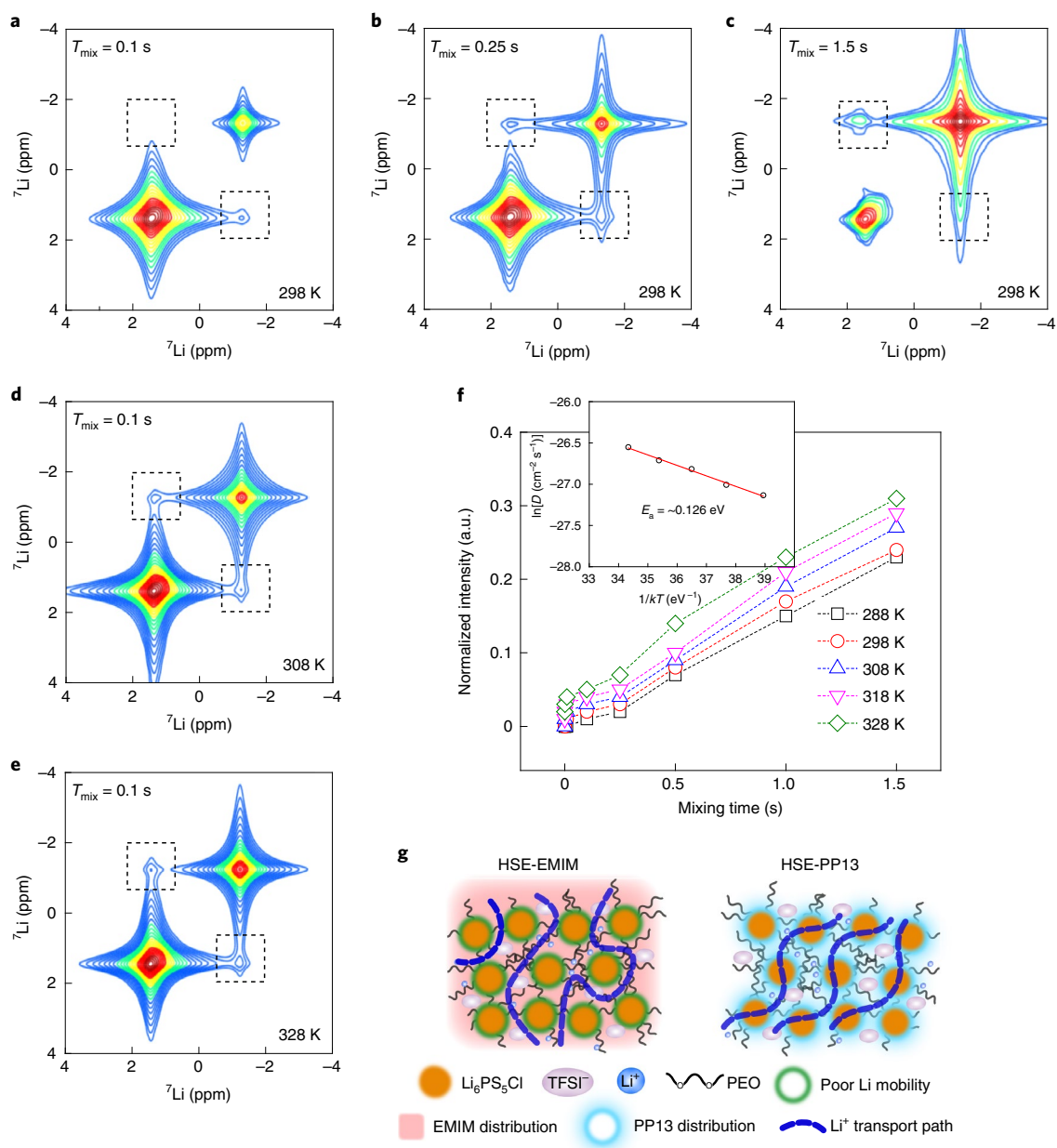
Fig. 5 | Quantification of Li-ion diffusion across phase boundaries in the HSE with the PP13-TFSI IL. a–e, 2D {}^7\text{Li} - {}^7\text{Li} EXSY spectra of the mixture of LiTFSI-PEO- \text{Li}_6\text{PS}_5\text{Cl} with PP13-TFSI IL measured at a spinning speed of 5 kHz at 298 K with mixing times T_{\text{mix}} of 0.1, 0.25 and 1.5 s ( a–c ) and at 308 K ( d ) and 328 K ( e ) with a T_{\text{mix}} of 0.1 s. f, Evolution of cross-peak intensity as a function of T_{\text{mix}} obtained from the 2D-EXSY measurements performed at the temperatures indicated in the graph. The line passing through the symbols is a guide to the eye. The inset figure is the dependence of the diffusion coefficient ( D ) obtained from fitting the data in f to a diffusion model described by us in detail elsewhere 30 . The normalized intensity is denoted in arbitrary units (a.u.). These can be fitted with the Arrhenius law, yielding an activation energy ( E_a ) of 0.126 eV. g, Proposed mechanism for Li-ion diffusion in HSEs with EMIM-TFSI and PP13-TFSI IL additives. Intensity from low to high is shown from blue to red in a–e .
