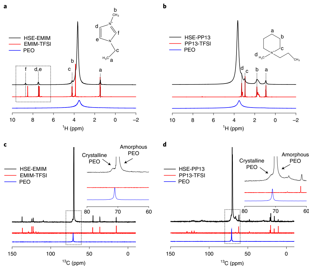
Fig. 3 | Structural characterization of the HSEs with PP13-TFSI and EMIM-TFSI IL additives. a, b , 1D ^1\text{H} spectra of LiTFSI-PEO- \text{Li}_6\text{PS}_5\text{Cl} HSEs with EMIM-TFSI (HSE-EMIM) and PP13-TFSI (HSE-PP13) ILs. ^1\text{H} spectra of PEO (solid), EMIM-TFSI (liquid) and PP13-TFSI (liquid) are included for comparison. c, d , ^{13}\text{C} CPMAS spectra of LiTFSI-PEO- \text{Li}_6\text{PS}_5\text{Cl} HSEs with EMIM-TFSI (HSE-EMIM) and PP13-TFSI (HSE-PP13) ILs. ^{13}\text{C} spectra of PEO (solid, CPMAS), EMIM-TFSI (liquid) and PP13-TFSI (liquid) are included for comparison.
