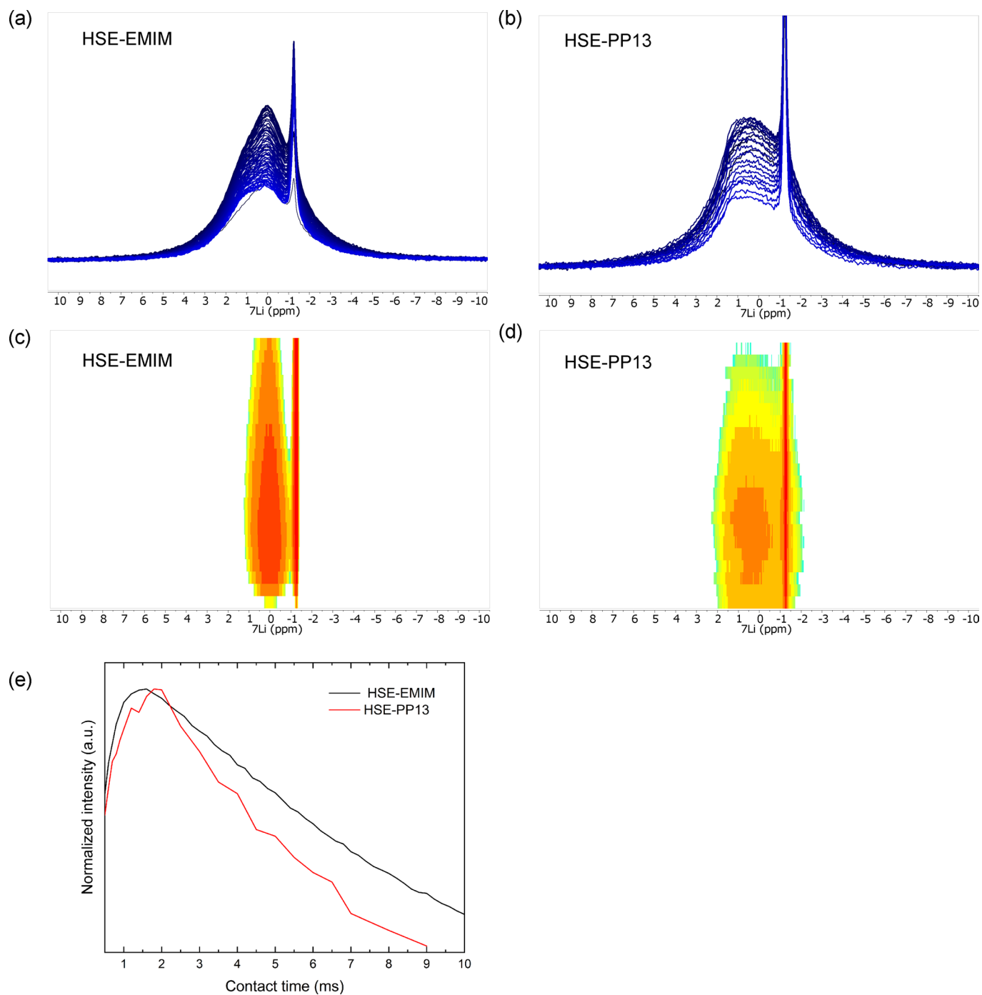
Extended Data Fig. 6 | ^7\text{Li} CPMAS spectra and intensity plots measured of the HSE-EMIM and HSE-PP13, and the full build-up of the peak intensity of the broad component. ^7\text{Li} CPMAS spectra and intensity plots measured of the (a,c) HSE-EMIM and (b,d) HSE-PP13 at contact times between 200\ \mu\text{s} and 12 ms (e) Full build-up of peak intensity at 0.2–0.7 ppm as function of contact time of the spectra given in (a) and (b).
