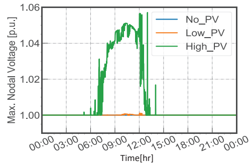
Fig. 11: Maximum nodal voltages for increasing EV penetration in different PV scenarios for sub urban grid
