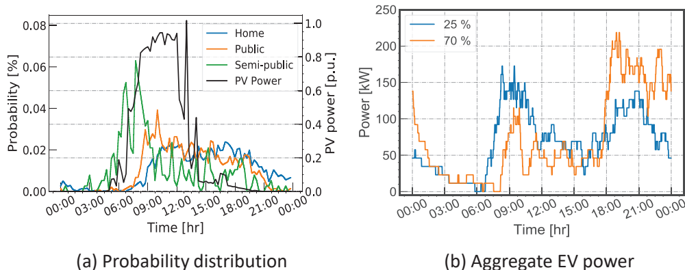
Fig. 2: (a) Probability distribution of EV arrival time for different charger types. (b) Aggregate EV power with respect to home charger variation.
