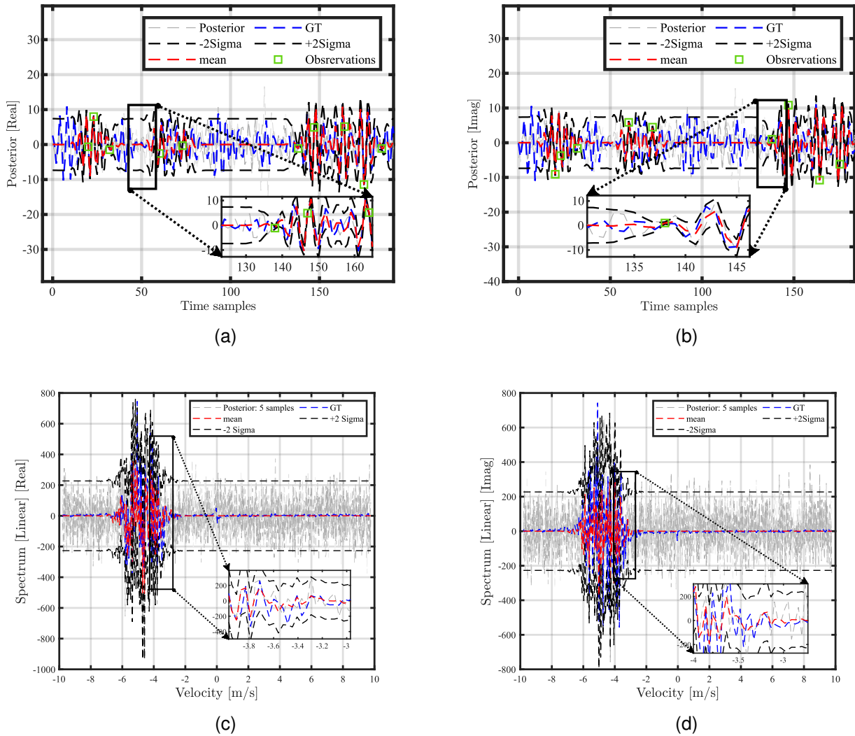
Fig. 2. Reconstruction in time and frequency domain (a) Real part of the time domain signal (b) Imaginary part of the signal in time domain (c) Real part of the local spectrum. (d) Imaginary part of the local spectrum.
