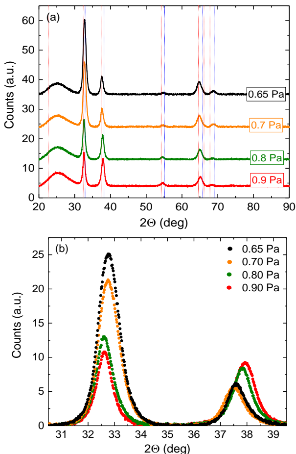
Figure A6.23. (a) Background subtracted XRD pattern of the ALD coated \text{NdO}_x\text{H}_y films prepared at different deposition pressures. (b) Detailed view showing the first two diffraction peaks of ALD coated films fabricated above the critical pressure.
