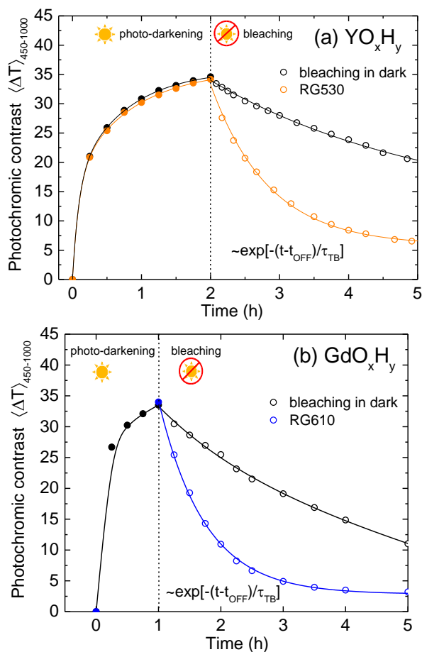
Figure 4.18. Analysis of optical bleaching kinetics on YO x H y and GdO x H y thin films (350 and 309 nm respectively grown above their critical pressure).
