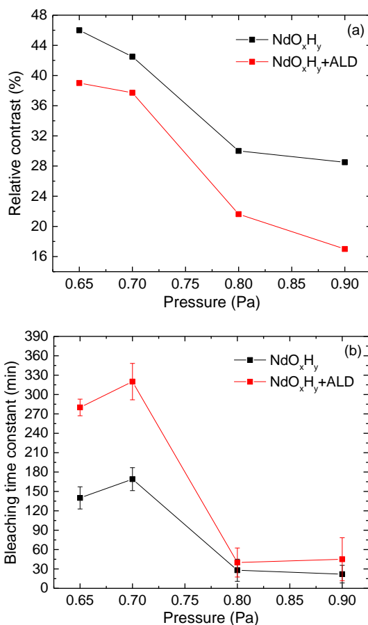
Figure 6.12. (a) The relative contrast and (b) bleaching time for as-deposited and ALD coated films as a function of deposition pressure obtained from the analysis of data shown in Figure 6.11.
