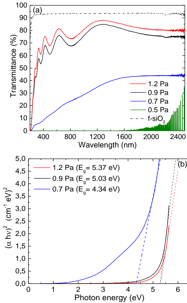
Figure 5.4. (a) UV-vis transmission spectra for Zr-based films prepared at different deposition conditions in Ar/H 2 atmosphere with thicknesses between 271 and 351 nm (b) calculated band gaps using Tauc plot for all samples
