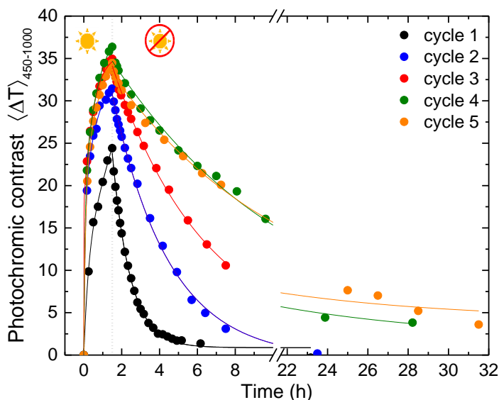
Figure 4.17. Multiple illumination cycles of 350 nm YO_xH_y thin film. Using a UV lamp at 5860 \mu W \text{ cm}^{-2} total irradiances for 90 min followed by thermal bleaching in the dark.
