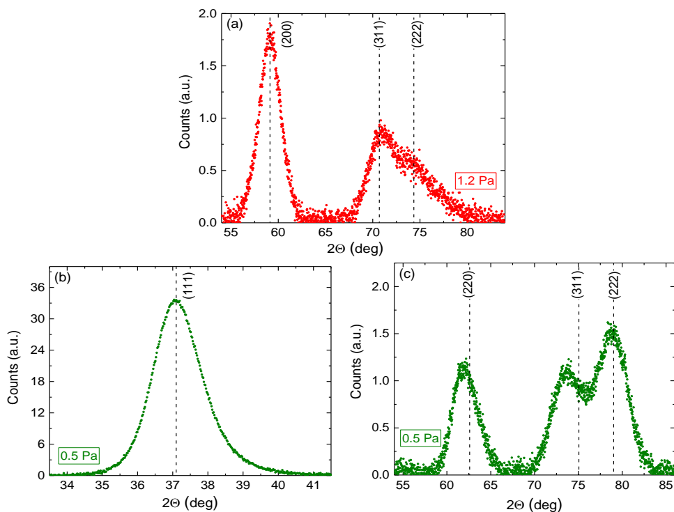
Figure 5.2. (a) narrow range XRD pattern of Zr-based films deposited at 1.2 Pa. The vertical dashed lines are peak positions corresponding to fcc- \text{ZrO}_2 ICDD PDF pattern #00-049-1642. (b&c) Narrow range diffraction pattern of the film prepared at 0.5 Pa. The vertical dashed lines are peak positions corresponding to fcc \delta\text{-ZrH}_{2-x} (ICDD-PDF pattern #01-071-4972) with a 1.7% expanded lattice constant of 4.87 Å to match (111) diffraction peak position.
