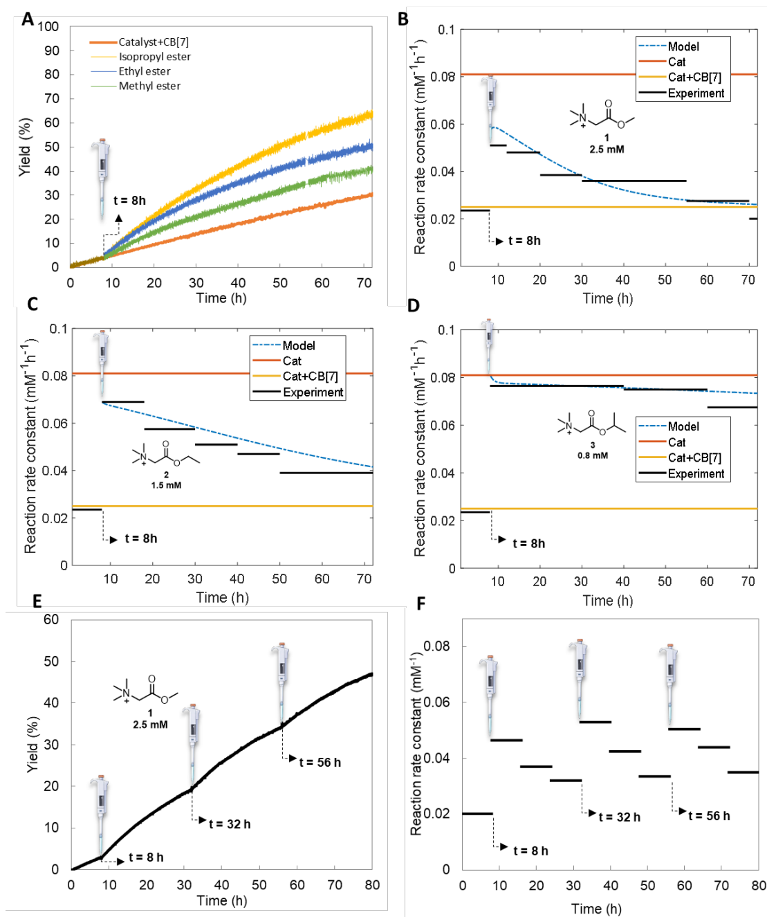
Figure 4: (A) Yield of hydrazone 9 for in-situ addition of esters 1-3 at t=8h. Rate constant for hydrazone formation as a function of time at various catalytic conditions. Experimental data with ester signals (black lines) are compared with the model (blue dashed line): (B) Methyl ester 1 2.5 mM, (C) Ethyl ester 2 1.5 mM and (D) Isopropyl ester 3 0.8 mM. Conditions: pH 7.5 100 mM phosphate buffer, 0.2 mM aldehyde 7 , 0.02 mM hydrazide 8 , 0.2 mM catalyst 6 and 0.6 mM CB[7], (E) Yield of hydrazone 9 and (F) Rate constant for hydrazone formation as a function of time for 3 consecutive additions of methyl ester ( 1 ) at t = 8 h, 32 h and 56 h. Conditions: pH 7.6 100 mM phosphate buffer, 2.5 mM methyl ester 1 ( \times 3 ), 0.2 mM aldehyde 7 , 0.02 mM hydrazide 8 , 0.2 mM catalyst 6 and 0.42 mM CB[7].
