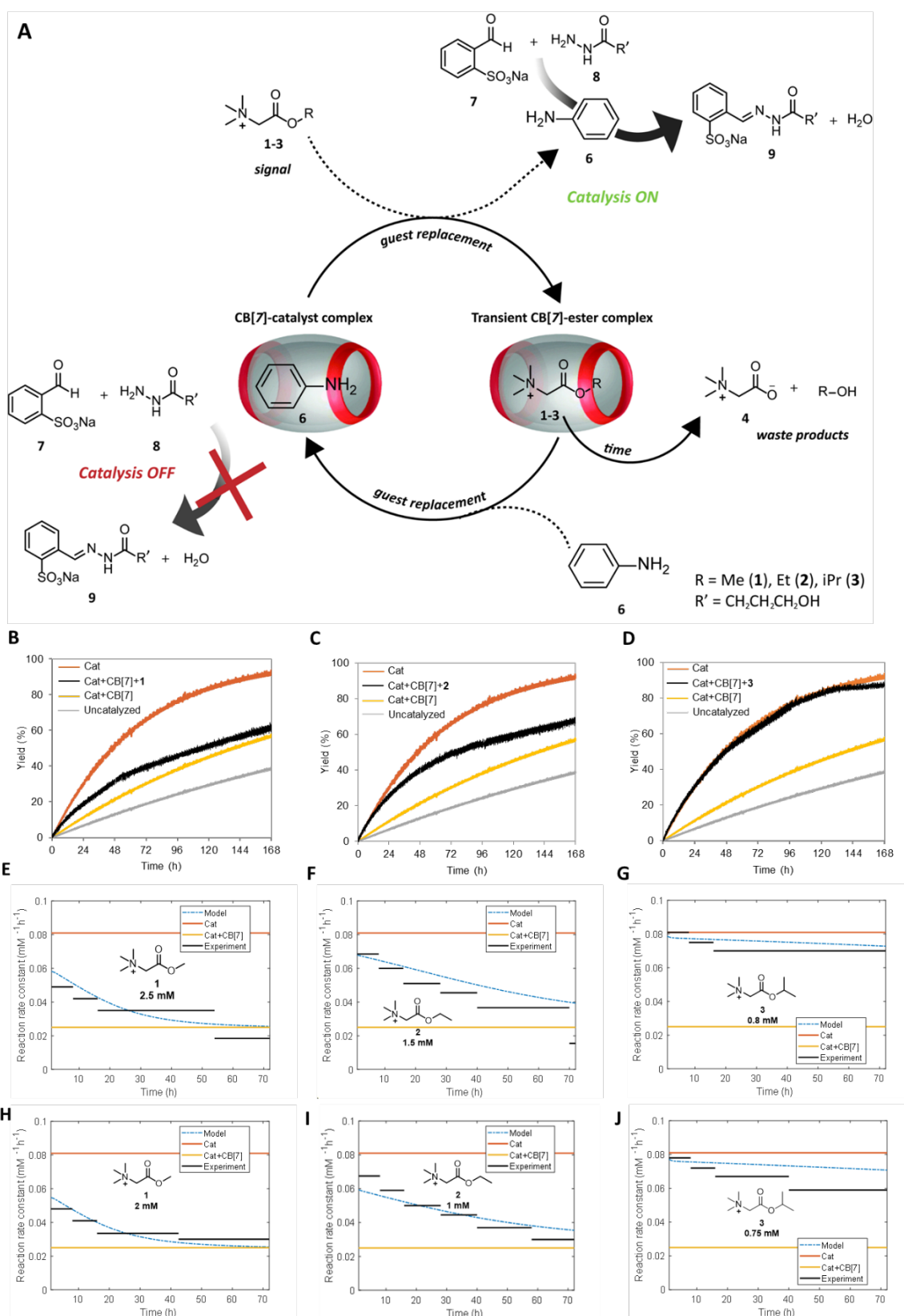
Figure 3: (A) Transient complex formation of hydrolysable ester signals with CB[7] to control the rate of hydrazone formation by aniline catalyst 6 capture and release. Yield (B-D) and rate constant (E-J) for hydrazone formation as a function of time at various catalytic conditions. Values extracted from experimental data with ester signals (black lines) are compared with the model (blue dashed line): (B,E) Methyl ester 1 2.5 mM, (C,F) Ethyl ester 2 1.5 mM, (D,G) Isopropyl ester 3 0.8 mM, (H) Methyl ester 1 2 mM, (I) Ethyl ester 2 1 mM and (J) Isopropyl ester 3 0.75 mM. Conditions: pH 7.5, 100 mM phosphate buffer; 0.2 mM aldehyde 7 , 0.02 mM hydrazide 8 , 0.2 mM catalyst 6 and 0.6 mM CB[7].
