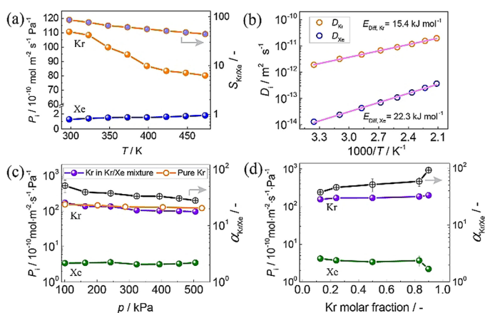
Figure 3. a,b) Single component permeation and diffusivity at different temperatures and 1.5 bar. c) Feed pressure-dependent Kr/Xe equimolar mixture separation performance at 298 K. d) Kr/Xe mixture separation performance for different compositions at 298 K and 1 bar. Membrane M2 was used.
