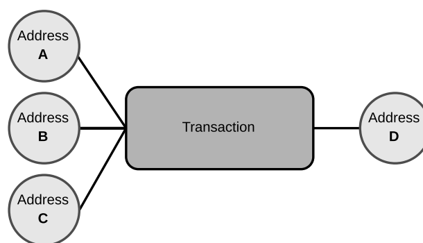
FIGURE 1. Bitcoin address co-spending heuristic: Example of three Bitcoin addresses with common spending in one transaction.
