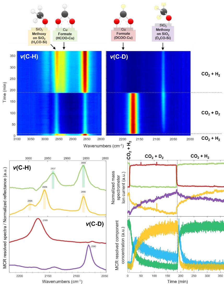
Figure S4.8 Transient responses of surface species and gas products during transient isotopic switching from \text{CO}_2+\text{D}_2 to \text{CO}_2+\text{H}_2 over Cu-In/SiO 2 . Time-resolved DRIFT spectra of \nu(\text{C-H}) region and \nu(\text{C-D}) region. Component spectra obtained by MCR were applied to the time-resolved DRIFT spectra. Concentration profiles of the spectra of the corresponding components obtained by MCR. Corresponding normalized ion current signal of isotope-labeled products. Reaction conditions: 10 mg catalyst, \text{H}_2(\text{or D}_2)/\text{CO}_2 = 3 , T = 230^\circ\text{C} , P = 10\text{ bar} , F_{\text{total}} = 10\text{ NmL min}^{-1}
