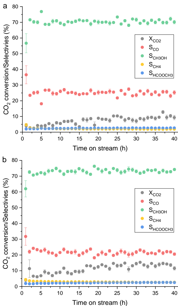
Figure 6.4: Catalytic stability during \text{CO}_2 hydrogenation of a Re(3)/TiO 2 and b Re(3)-Ag(1)/TiO 2 . Reaction conditions: T = 150 °C, P = 60 bar, \text{H}_2/\text{CO}_2 = 3 , SV = 3505 NmL g cat -1 h -1 .
