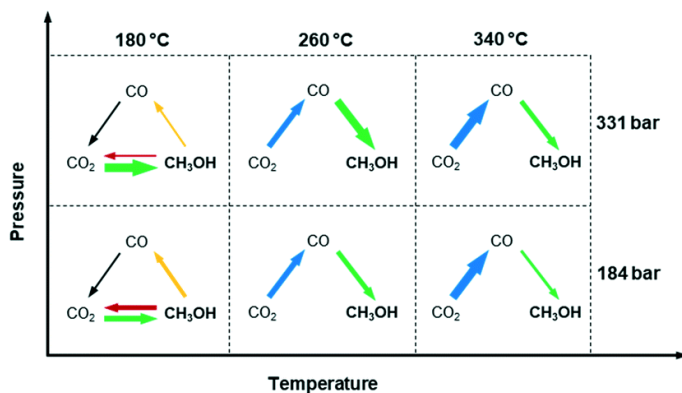
Figure 3.5 Major reaction pathways in high-pressure \text{CO}_2 hydrogenation over \text{Cu/ZnO/Al}_2\text{O}_3 catalyst at 180 °C, 260 °C, and 340 °C at 184 and 331 bar. The width of the arrow shows the amount of one species' transformation to others.
