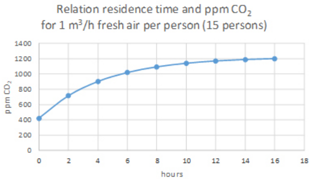
a. CO 2 -concentration for 15 persons with 25m 3 /h pp air supply in relation to time
