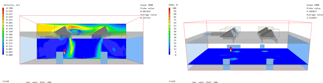
c. Air velocities d. Draught Rate Values at 1.1 m CFD-Draught risk analysis of natural ventilation with rooftop windows at an outside temperature of 15 °C. Window-opening 40 cm. Fresh air supply sufficient for 24 persons.
