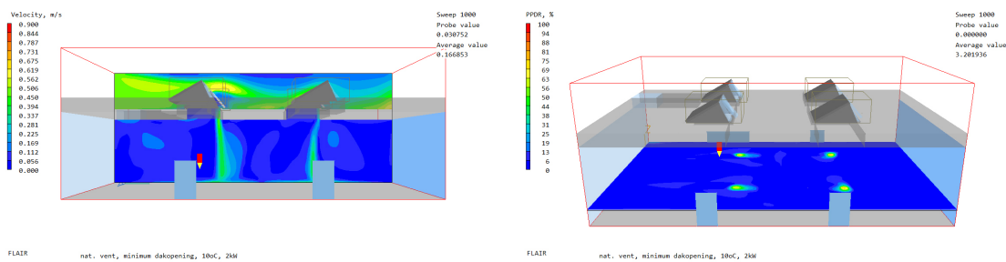
a. Air velocities b. Draught Rate Values at 1.1 m CFD-Draught risk analysis of natural ventilation with rooftop windows at an outside temperature of 10 °C. Window-opening 10 cm. Fresh air supply sufficient for 15 persons.
