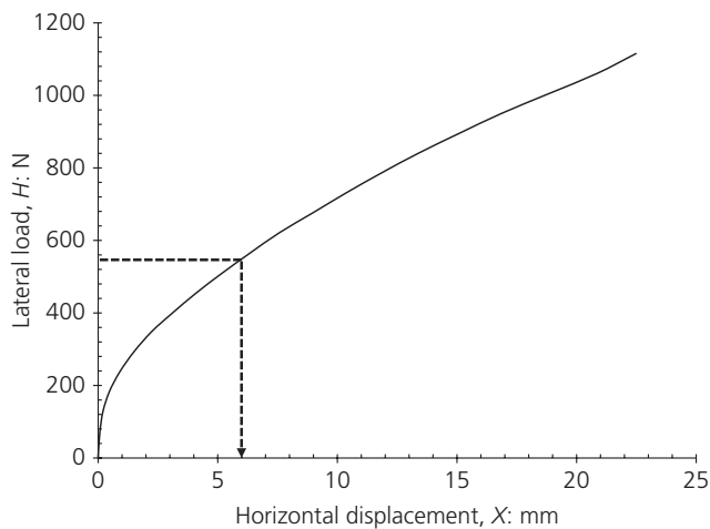
Figure 5. Control test, monotonic loading ( T_0 )
