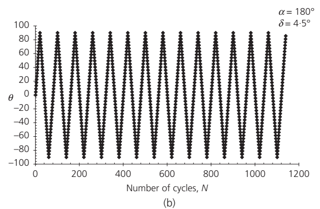
Figure 2. (a) Multi-directional loading direction. (b) The \theta-N used in this investigation
