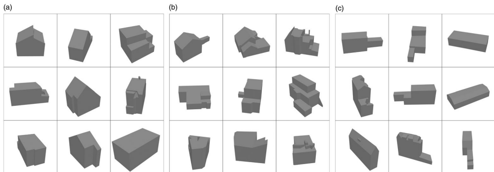
Figure 12. The three largest clusters of the hierarchical clustering analysis conducted on a sample of 200,000 buildings based on the 3D indices. The clustering input was eleven features based on principal components that represented the original 3D indices. We used the average linkage method to classify buildings in 30 clusters. These three clusters represent 86%, 7% and 4% of the sample, respectively. Clusters (a) and (b) are very similar, although on average objects in the latter seem to be slightly more complex. Cluster (c) portrays more elongated objects, mostly with protrusions.
