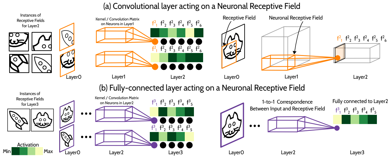
Fig. 3. In deeper layers, filter functions are trained to detect more complex patterns in larger receptive fields. In convolutional layers a subset of the neurons in the previous layer, the neuronal receptive field, is the input to the filter functions rather than the receptive field instance (a). The same description holds for a fully-connected layer, however, it differs from convolutional layers as the receptive field of a neuron corresponds to the complete input and the neuronal receptive field contains all the neurons in the previous layer (b).
