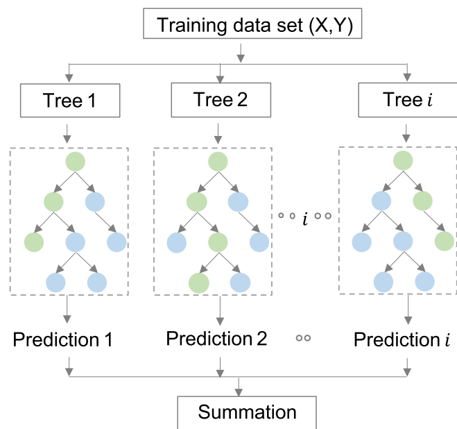
Fig. 9. General working flow of random forest algorithm.
