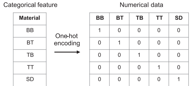
Fig. 7. One-hot encoding of epoxy polymer “Material” feature.
