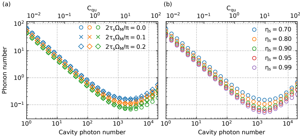
Figure 5.4: Coherent feedback with delay for (a) an auxiliary cavity and (b) an auxiliary mirror. In (a), the round trip delay are 0, 0.05 and 0.1 \mu s, corresponding to a feedback phase 2\Omega_M\tau_s of 0, 0.1\pi and 0.2\pi . The single way efficiency over the optical path is \eta_s = 0.7, 0.8, 0.9 for blue, orange and green curves. The phonon number is minimized numerically with respect to \kappa_A^{(1)} , \Delta_A and \phi_s . In (b), the reflectivity of the auxiliary mirror is set to 1. Non-unity reflectivity can be included in the optical path efficiency. The phonon number is minimized with respect to \tau_s and \phi_s .
