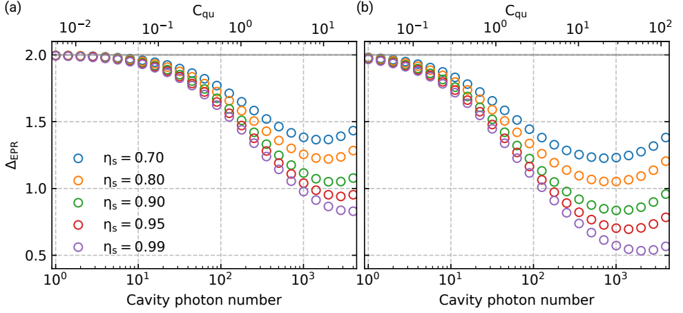
Figure 5.7: Optimized \Delta_{\text{EPR}} for (a) Q_M = 2 \times 10^7 and (b) Q_M = 10^8 . The gray solid line shows the separability bound \Delta_{\text{EPR}} = 2 .
