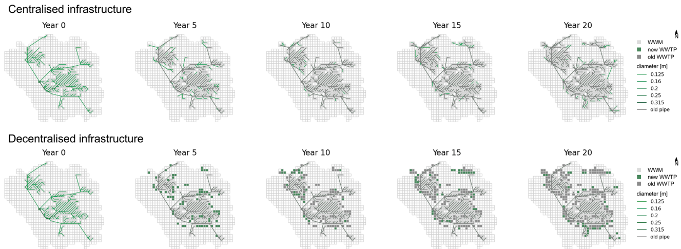
Fig. 5. Wastewater infrastructure expansion to connect the new development areas. The maps include the layout of the sewer pipes and WWTPs and the corresponding hydraulic design for centralised (top) and decentralised (bottom) alternatives in the case study. New infrastructure is highlighted in colour, while old infrastructure appears in grey. .
