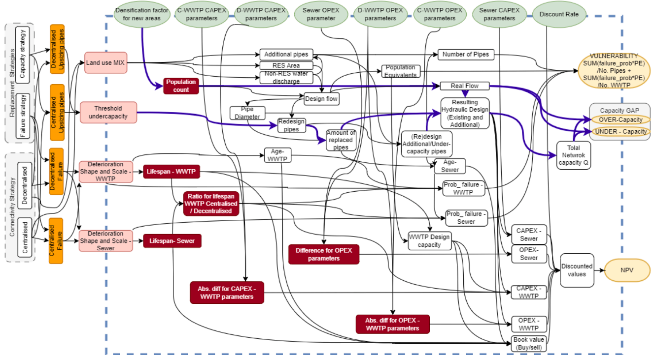
Fig. A.2. System diagram for the network's hydraulic capacity index.
