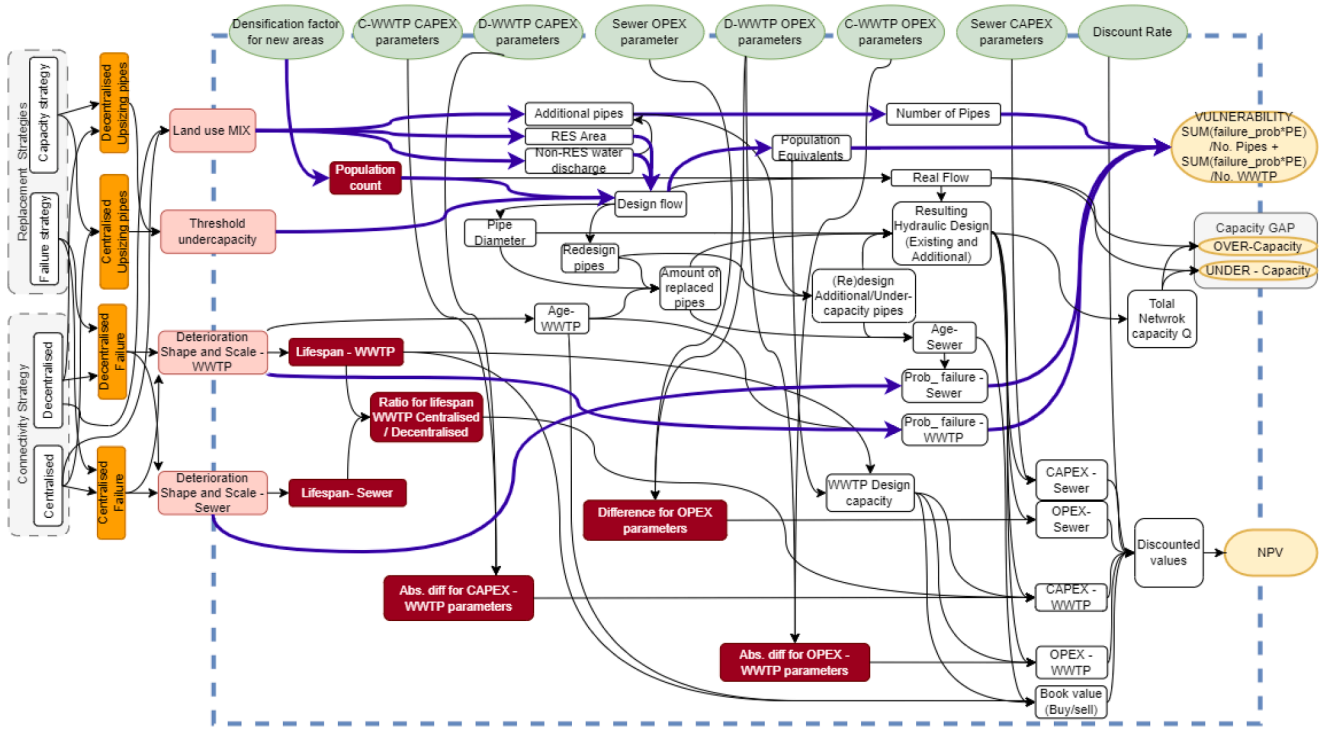
Fig. A.1. System diagram for the structural vulnerability index.
