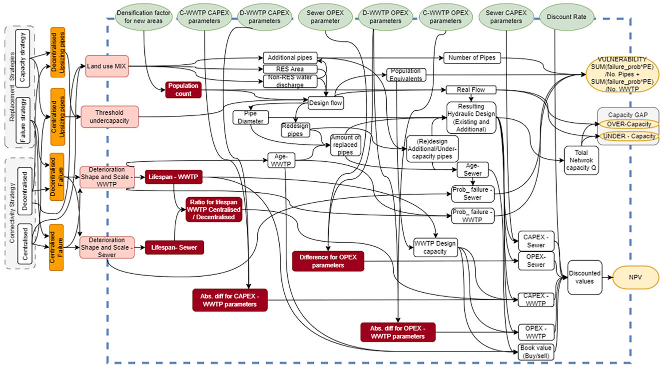
Fig. 3. System diagram for TURN-Sewers Model.
