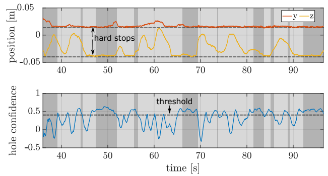
Fig. 10: Lateral TCP motion on y-z axes (top plot) in a sample experiment where the TCP movement is purposely blocked by hard stops (dashed lines). The light gray areas indicate the Search Pattern states, while the dark gray areas indicate the Hole Test state. The bottom plot shows the hole confidence \alpha_h and the corresponding threshold \alpha_{h,\text{thresh}} being responsible for the transition between the two states.
