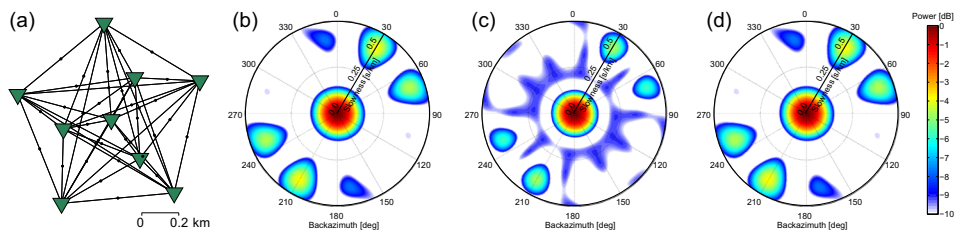
Fig. 3 a The configuration of array elements ( green triangles ) of the SPITS array (Fig. 1) and b–d corresponding ARFs for varying beamforming implementations, for a plane-wave source with p_S = 0 and f = 5 Hz. ARF for b conventional
