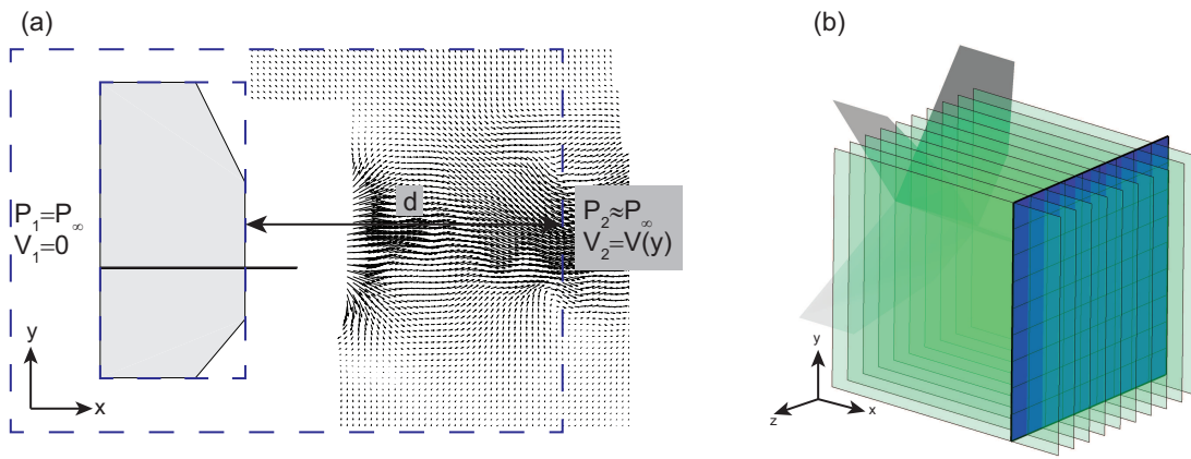
Fig. 16 a) Boundaries of the control volume ( dashed blue ) used for the estimation of the aerodynamic forces in a side view, b) streamwise oriented measurement planes ( green ) and downstream surface of the control volume ( blue ) formed from the velocity vectors of the measurement planes at 2.5\bar{c} streamwise distance from the trailing edge
