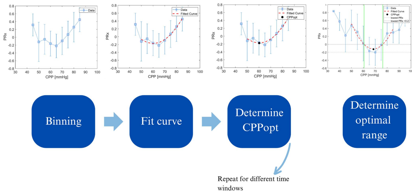
Fig. 1 Schematic overview of the CPPopt algorithm. In windows of one, two, four, six and eight hours, CPPopt was defined as the local minimum of a second order curve fitted along binned CPP and corresponding mean PRx. The optimal CPP range was determined from the corresponding optimal PRx range in the eight hour window between
