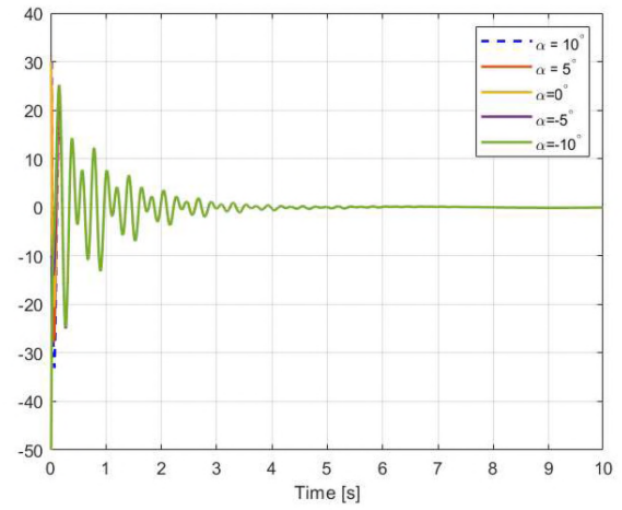
Fig. 6. Elevator Deflection.
